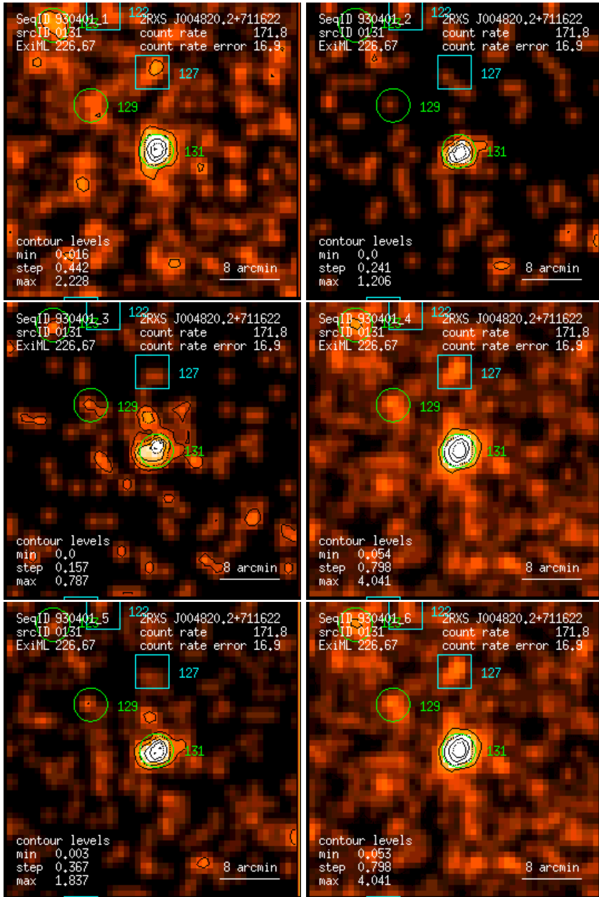
Figure 131: RASS 930401: detection 0131: band rate images, Gaussian filter: (1) PSPC channels 11 – 41, (2) 52 – 90, (3) 91 – 201, (4) 11 – 235, (5) 52 – 201, (6) 11 – 201. Broad band rates in counts/ks. Band rate contour levels in counts/ks/arcmin 2 .
