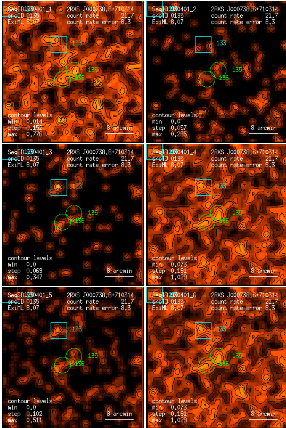
Figure 135: RASS 930401: detection 0135: band rate images, Gaussian filter: (1) PSPC channels 11 – 41, (2) 52 – 90, (3) 91 – 201, (4) 11 – 235, (5) 52 – 201, (6) 11 – 201. Broad band rates in counts/ks. Band rate contour levels in counts/ks/arcmin 2 .
