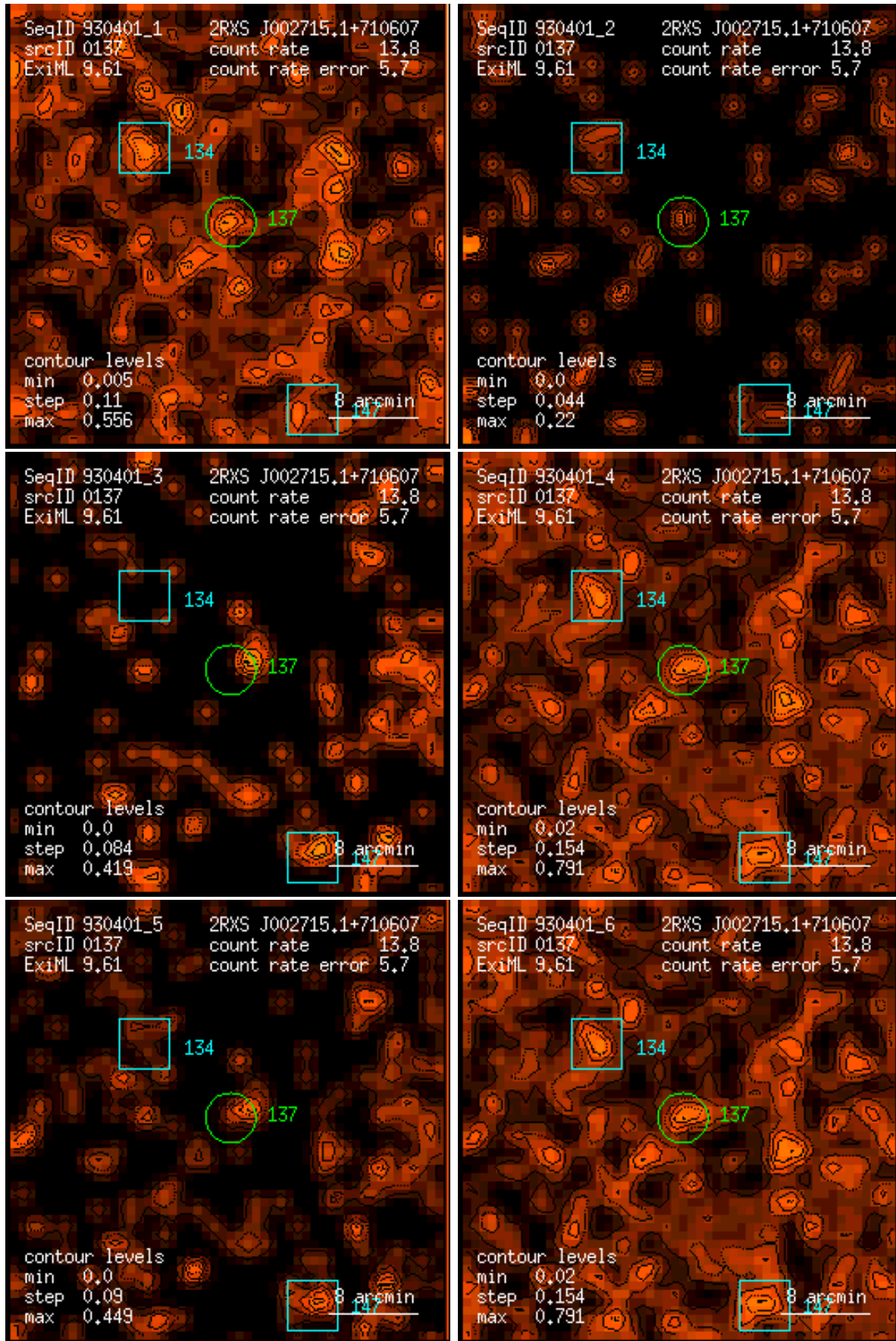
Figure 137: RASS 930401: detection 0137: band rate images, Gaussian filter: (1) PSPC channels 11 – 41, (2) 52 – 90, (3) 91 – 201, (4) 11 – 235, (5) 52 – 201, (6) 11 – 201. Broad band rates in counts/ks. Band rate contour levels in counts/ks/arcmin 2 .
