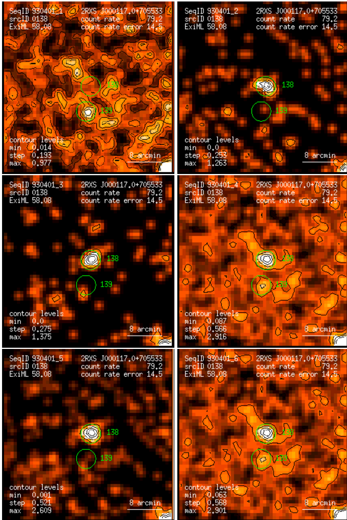
Figure 138: RASS 930401: detection 0138: band rate images, Gaussian filter: (1) PSPC channels 11 – 41, (2) 52 – 90, (3) 91 – 201, (4) 11 – 235, (5) 52 – 201, (6) 11 – 201. Broad band rates in counts/ks. Band rate contour levels in counts/ks/arcmin 2 .
