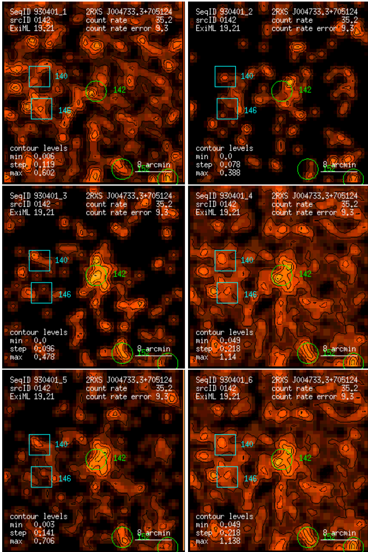
Figure 142: RASS 930401: detection 0142: band rate images, Gaussian filter: (1) PSPC channels 11 – 41, (2) 52 – 90, (3) 91 – 201, (4) 11 – 235, (5) 52 – 201, (6) 11 – 201. Broad band rates in counts/ks. Band rate contour levels in counts/ks/arcmin 2 .
