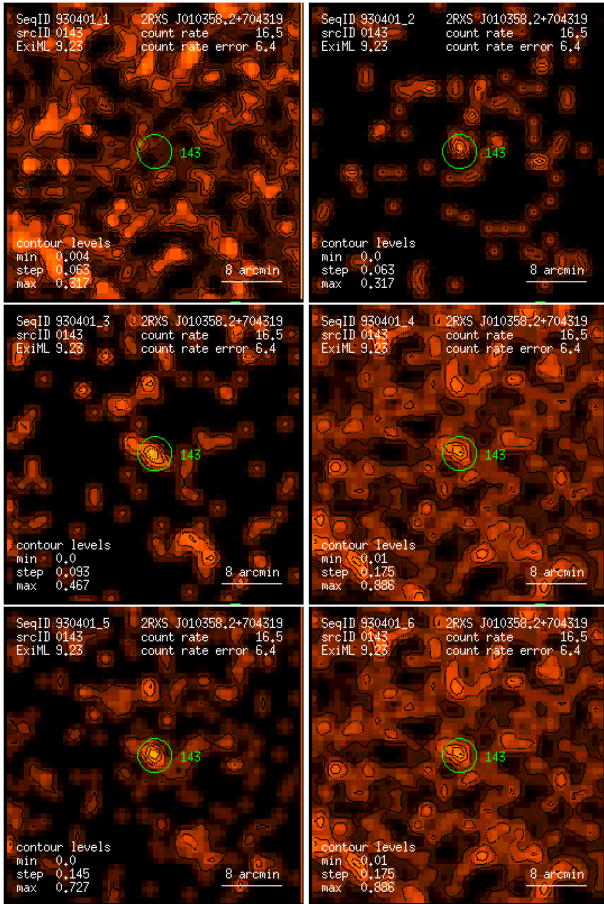
Figure 143: RASS 930401: detection 0143: band rate images, Gaussian filter: (1) PSPC channels 11 – 41, (2) 52 – 90, (3) 91 – 201, (4) 11 – 235, (5) 52 – 201, (6) 11 – 201. Broad band rates in counts/ks. Band rate contour levels in counts/ks/arcmin 2 .
