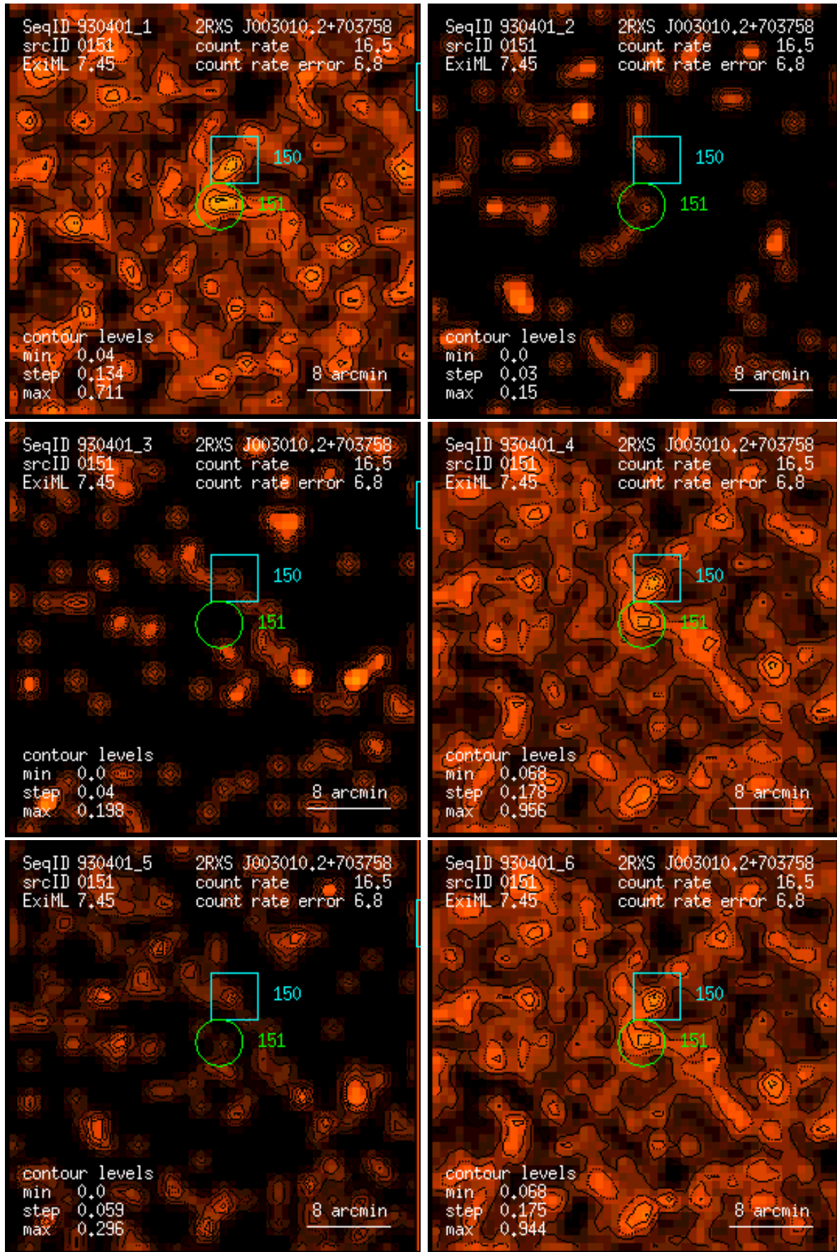
Figure 151: RASS 930401: detection 0151: band rate images, Gaussian filter: (1) PSPC channels 11 – 41, (2) 52 – 90, (3) 91 – 201, (4) 11 – 235, (5) 52 – 201, (6) 11 – 201. Broad band rates in counts/ks. Band rate contour levels in counts/ks/arcmin 2 .
