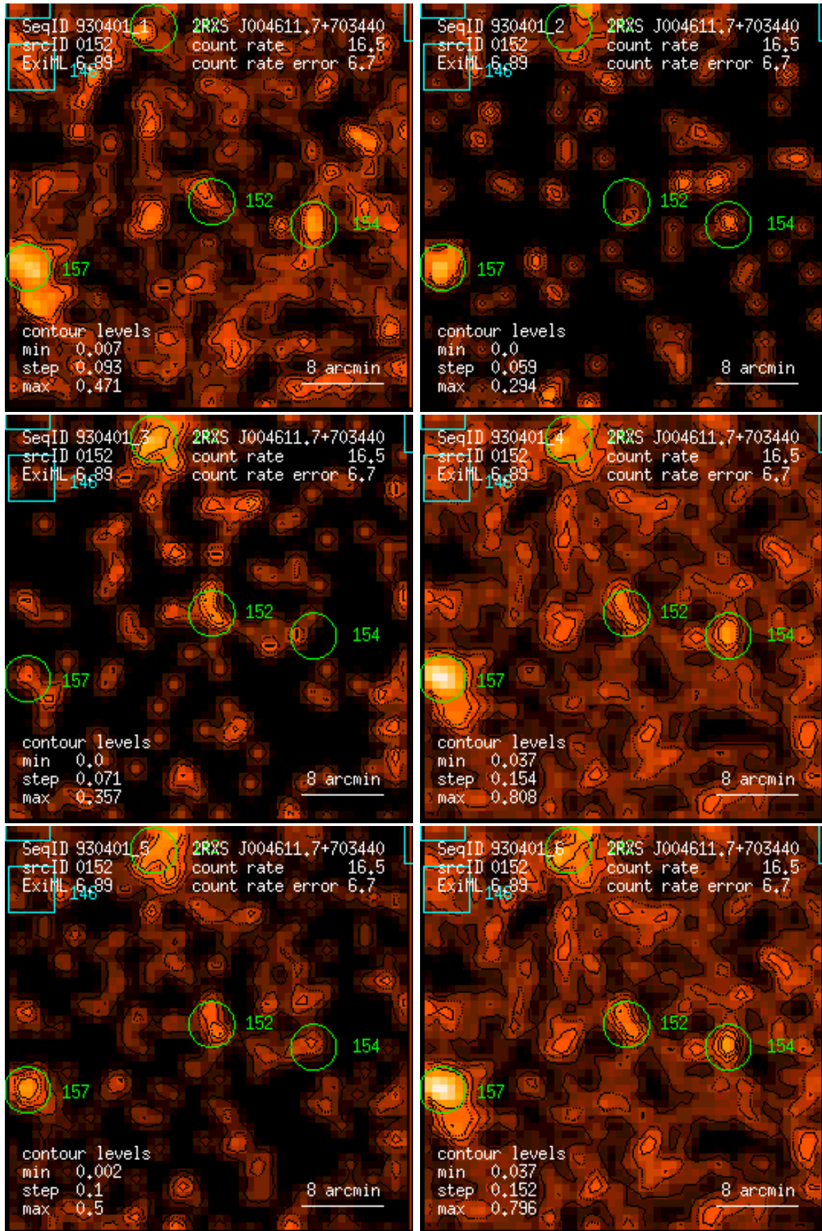
Figure 152: RASS 930401: detection 0152: band rate images, Gaussian filter: (1) PSPC channels 11 – 41, (2) 52 – 90, (3) 91 – 201, (4) 11 – 235, (5) 52 – 201, (6) 11 – 201. Broad band rates in counts/ks. Band rate contour levels in counts/ks/arcmin 2 .
