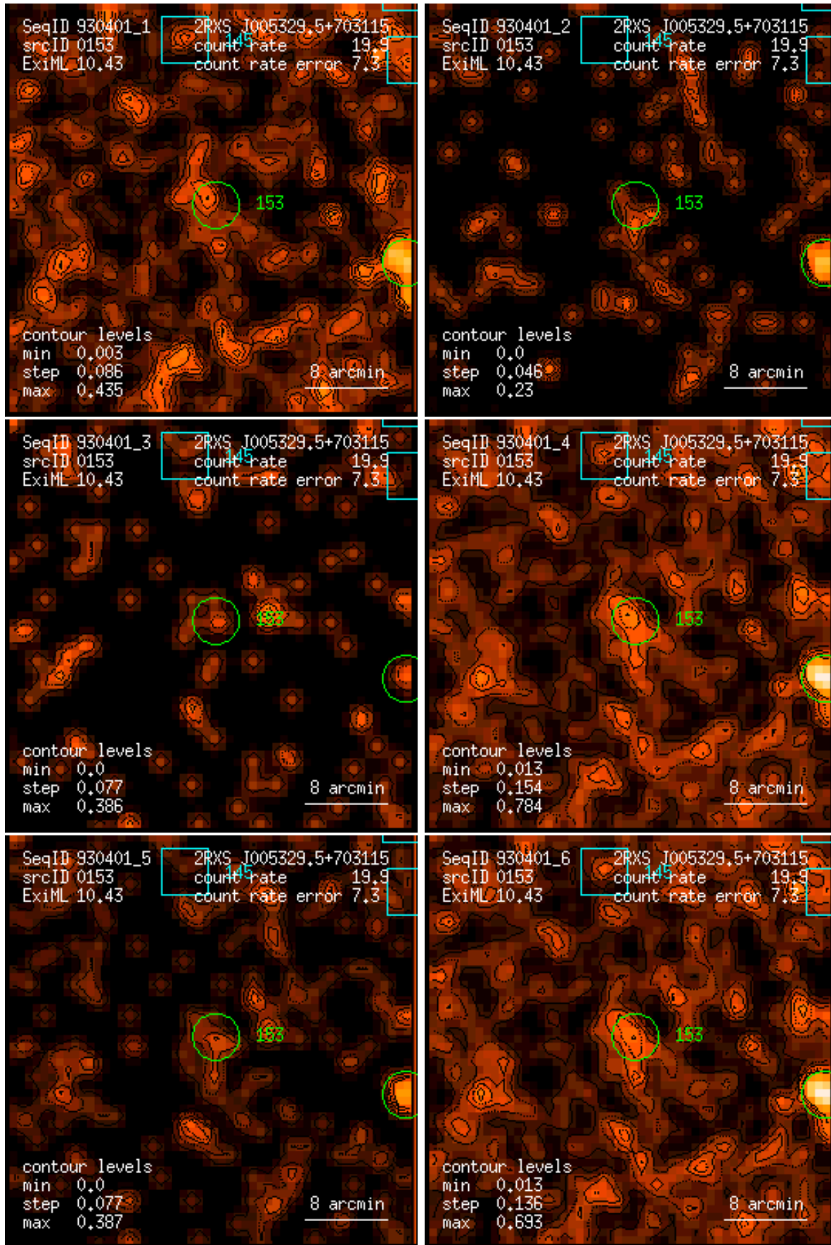
Figure 153: RASS 930401: detection 0153: band rate images, Gaussian filter: (1) PSPC channels 11 – 41, (2) 52 – 90, (3) 91 – 201, (4) 11 – 235, (5) 52 – 201, (6) 11 – 201. Broad band rates in counts/ks. Band rate contour levels in counts/ks/arcmin 2 .
