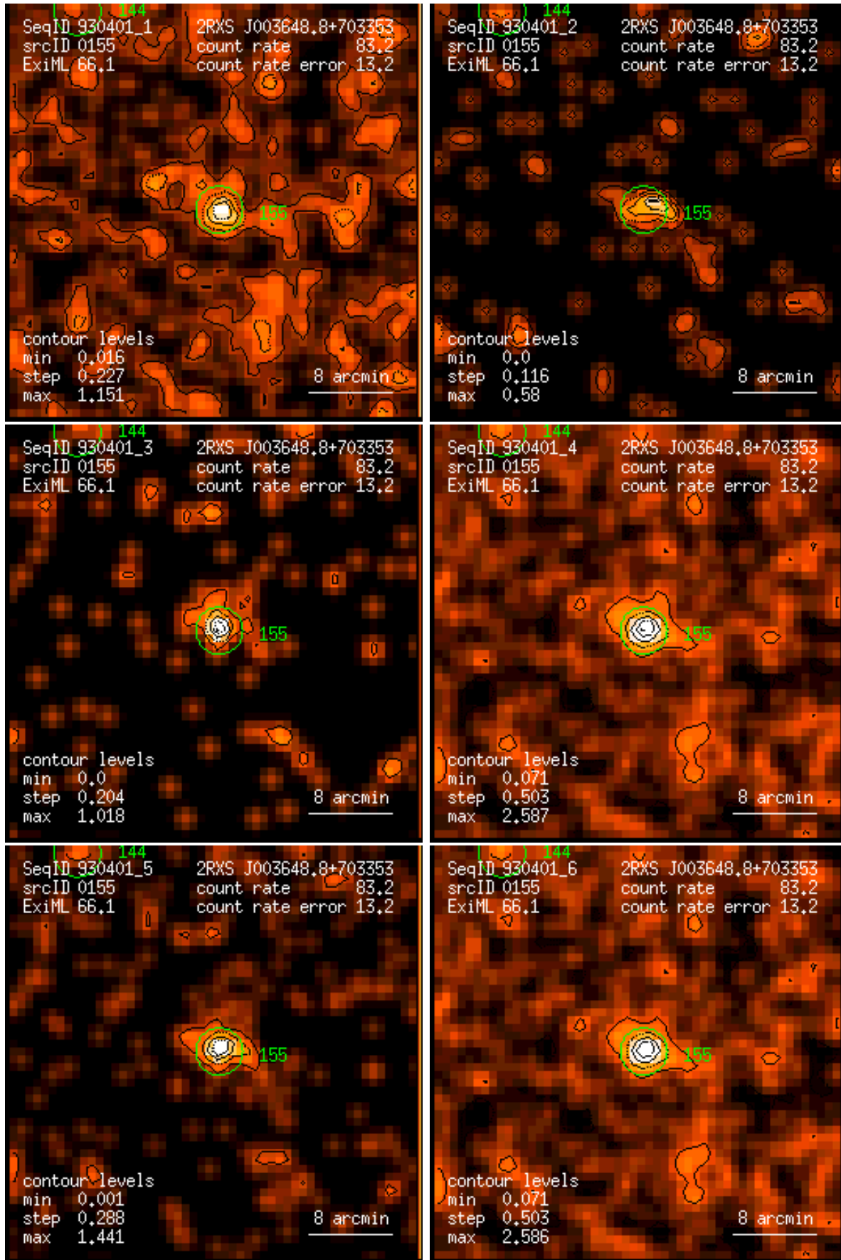
Figure 155: RASS 930401: detection 0155: band rate images, Gaussian filter: (1) PSPC channels 11 – 41, (2) 52 – 90, (3) 91 – 201, (4) 11 – 235, (5) 52 – 201, (6) 11 – 201. Broad band rates in counts/ks. Band rate contour levels in counts/ks/arcmin 2 .
