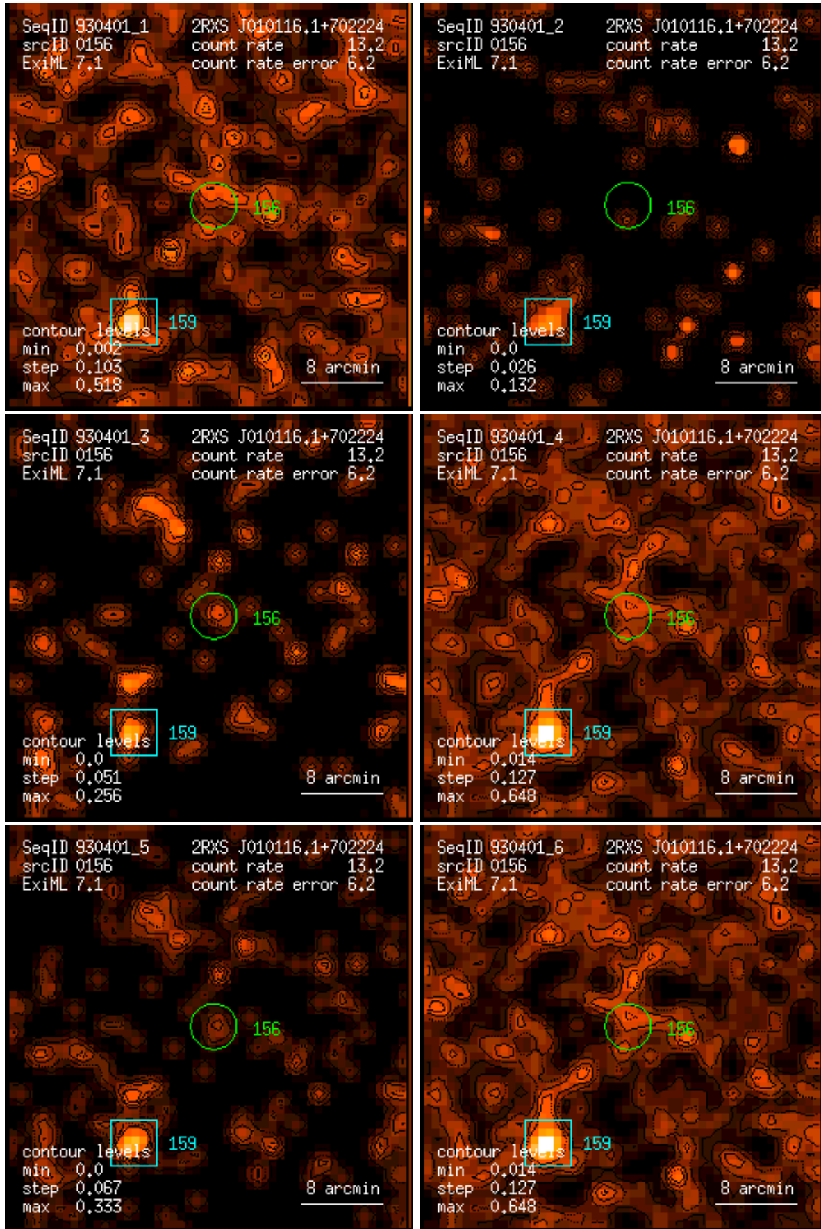
Figure 156: RASS 930401: detection 0156: band rate images, Gaussian filter: (1) PSPC channels 11 – 41, (2) 52 – 90, (3) 91 – 201, (4) 11 – 235, (5) 52 – 201, (6) 11 – 201. Broad band rates in counts/ks. Band rate contour levels in counts/ks/arcmin 2 .
