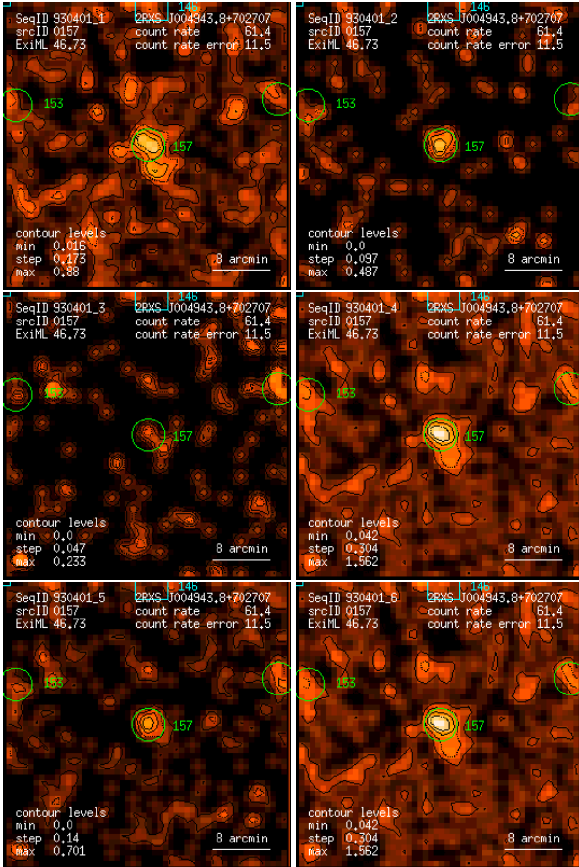
Figure 157: RASS 930401: detection 0157: band rate images, Gaussian filter: (1) PSPC channels 11 – 41, (2) 52 – 90, (3) 91 – 201, (4) 11 – 235, (5) 52 – 201, (6) 11 – 201. Broad band rates in counts/ks. Band rate contour levels in counts/ks/arcmin 2 .
