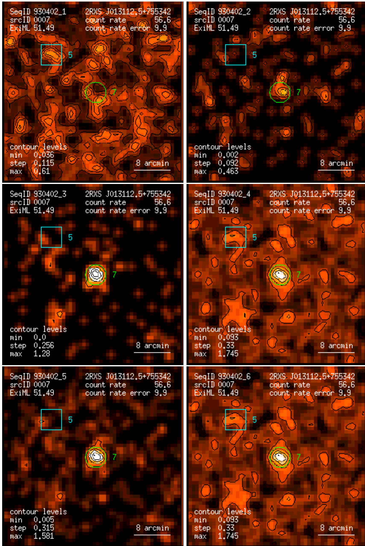
Figure 7: RASS 930402: detection 0007: band rate images, Gaussian filter: (1) PSPC channels 11 – 41, (2) 52 – 90, (3) 91 – 201, (4) 11 – 235, (5) 52 – 201, (6) 11 – 201. Broad band rates in counts/ks. Band rate contour levels in counts/ks/arcmin 2 .
