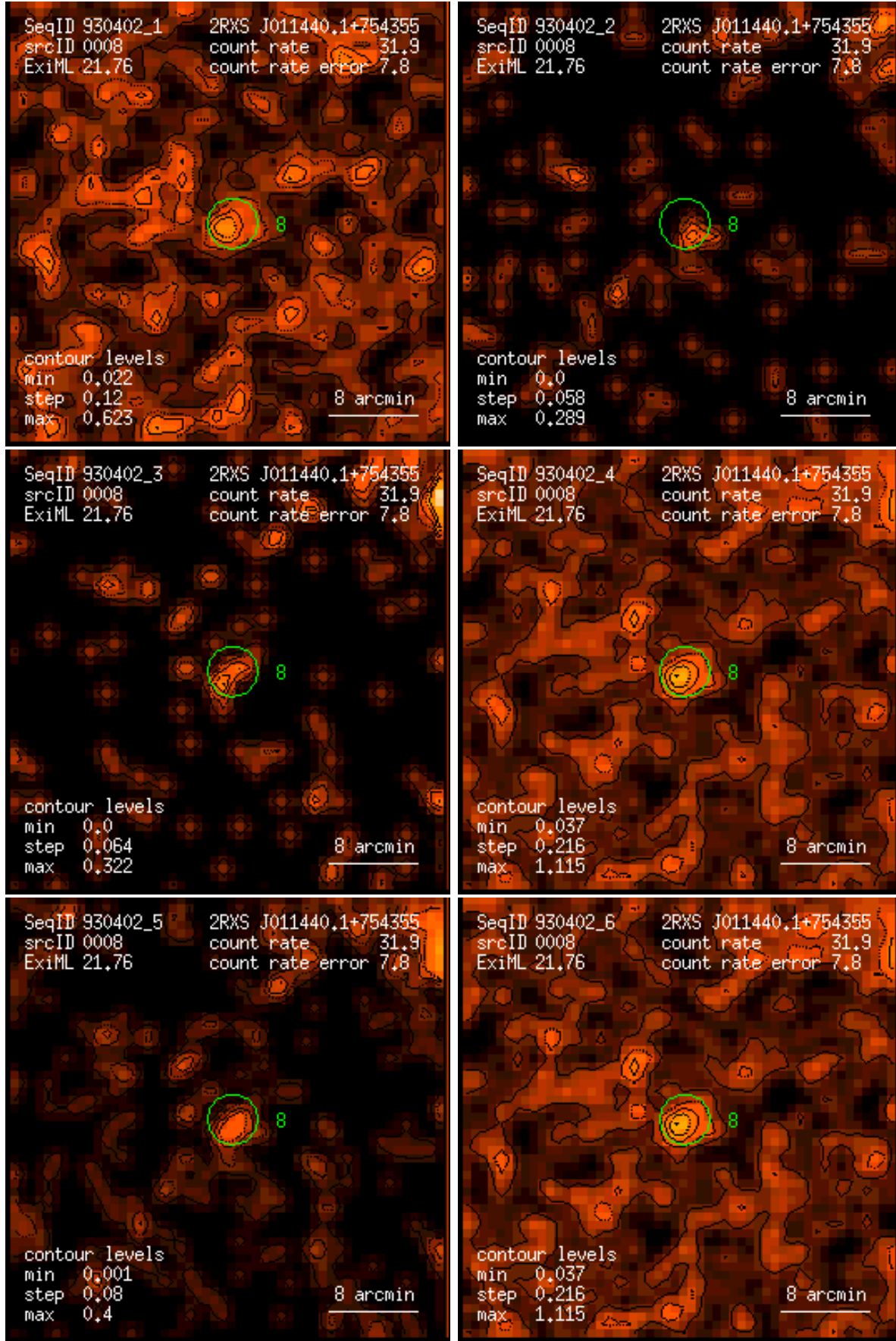
Figure 8: RASS 930402: detection 0008: band rate images, Gaussian filter: (1) PSPC channels 11 – 41, (2) 52 – 90, (3) 91 – 201, (4) 11 – 235, (5) 52 – 201, (6) 11 – 201. Broad band rates in counts/ks. Band rate contour levels in counts/ks/arcmin 2 .
