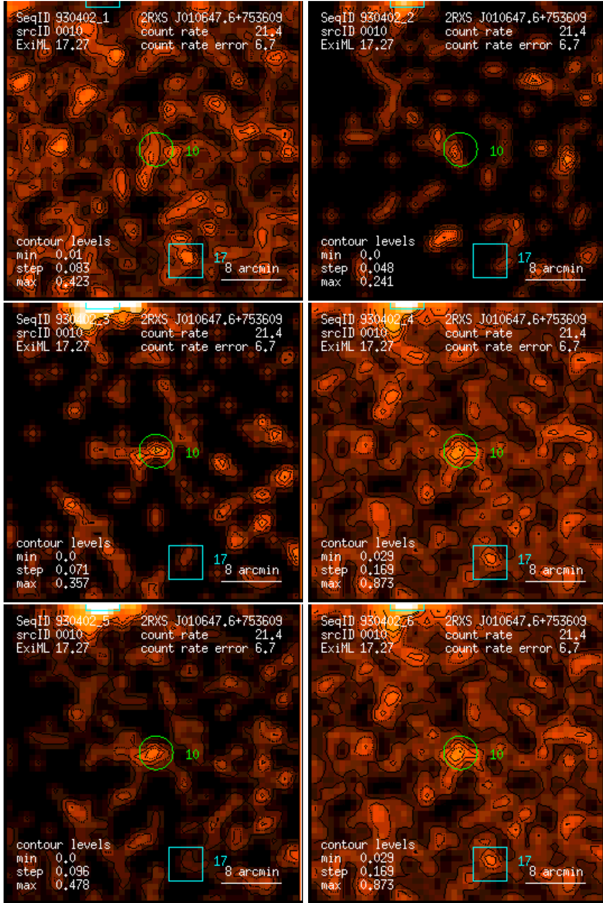
Figure 10: RASS 930402: detection 0010: band rate images, Gaussian filter: (1) PSPC channels 11 – 41, (2) 52 – 90, (3) 91 – 201, (4) 11 – 235, (5) 52 – 201, (6) 11 – 201. Broad band rates in counts/ks. Band rate contour levels in counts/ks/arcmin 2 .
