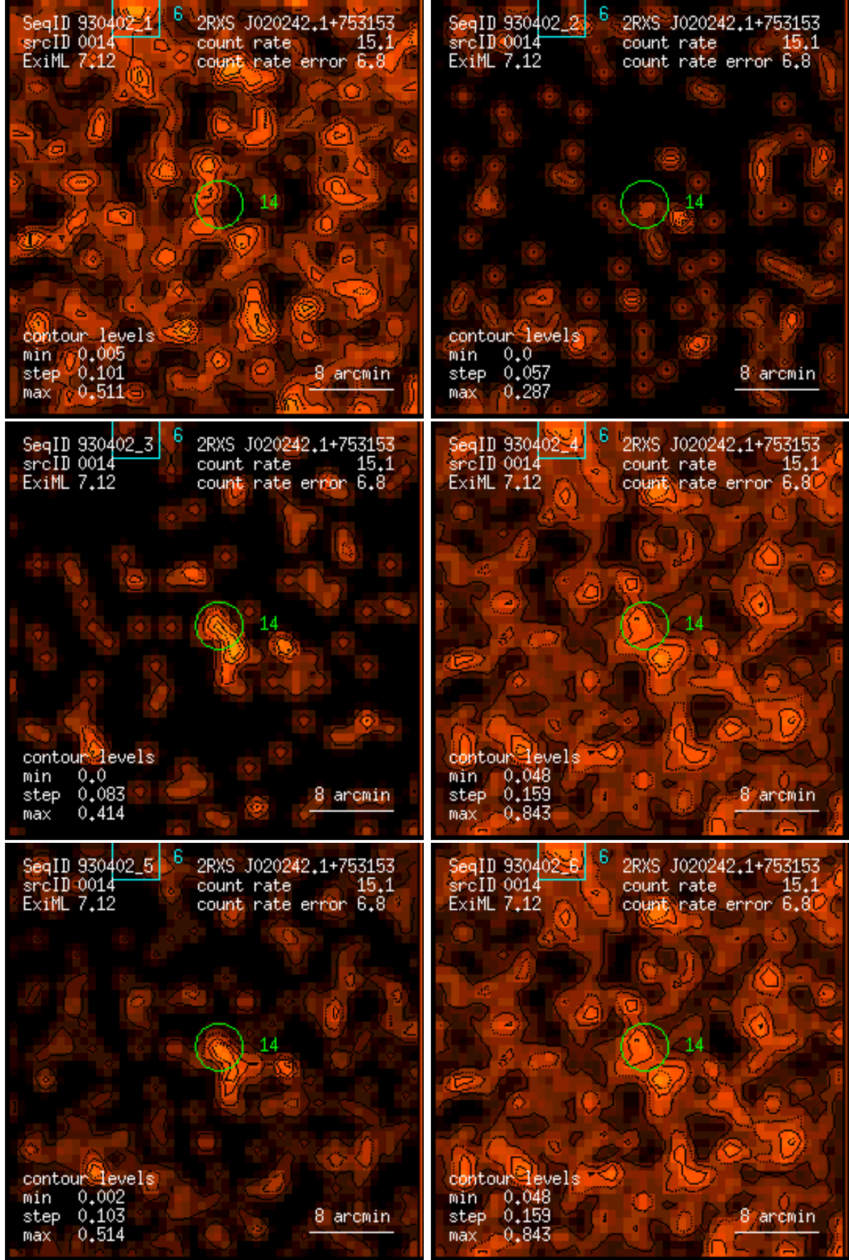
Figure 14: RASS 930402: detection 0014: band rate images, Gaussian filter: (1) PSPC channels 11 – 41, (2) 52 – 90, (3) 91 – 201, (4) 11 – 235, (5) 52 – 201, (6) 11 – 201. Broad band rates in counts/ks. Band rate contour levels in counts/ks/arcmin 2 .
