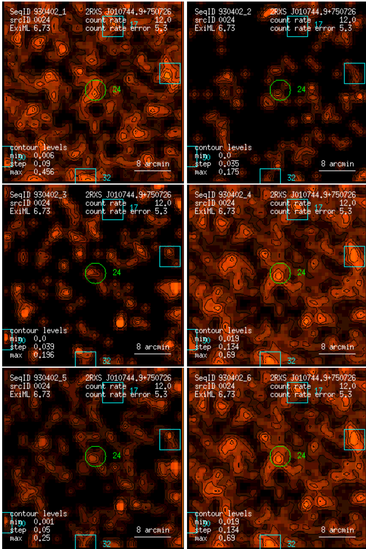
Figure 24: RASS 930402: detection 0024: band rate images, Gaussian filter: (1) PSPC channels 11 – 41, (2) 52 – 90, (3) 91 – 201, (4) 11 – 235, (5) 52 – 201, (6) 11 – 201. Broad band rates in counts/ks. Band rate contour levels in counts/ks/arcmin 2 .
