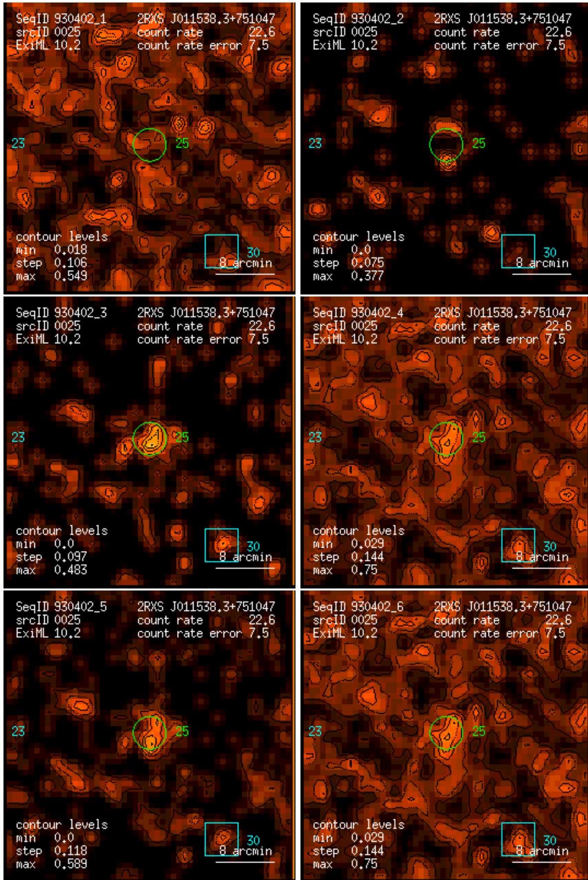
Figure 25: RASS 930402: detection 0025: band rate images, Gaussian filter: (1) PSPC channels 11 – 41, (2) 52 – 90, (3) 91 – 201, (4) 11 – 235, (5) 52 – 201, (6) 11 – 201. Broad band rates in counts/ks. Band rate contour levels in counts/ks/arcmin 2 .
