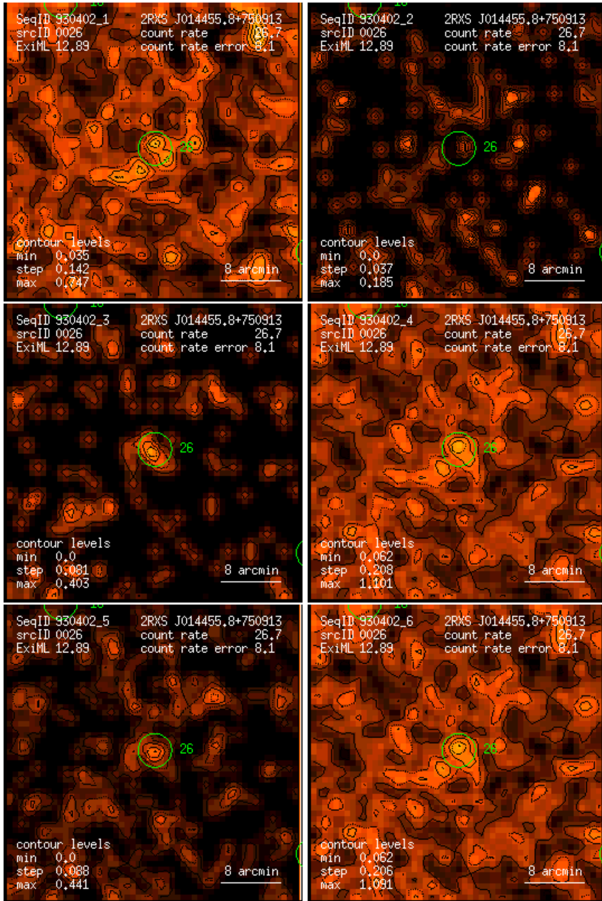
Figure 26: RASS 930402: detection 0026: band rate images, Gaussian filter: (1) PSPC channels 11 – 41, (2) 52 – 90, (3) 91 – 201, (4) 11 – 235, (5) 52 – 201, (6) 11 – 201. Broad band rates in counts/ks. Band rate contour levels in counts/ks/arcmin 2 .
