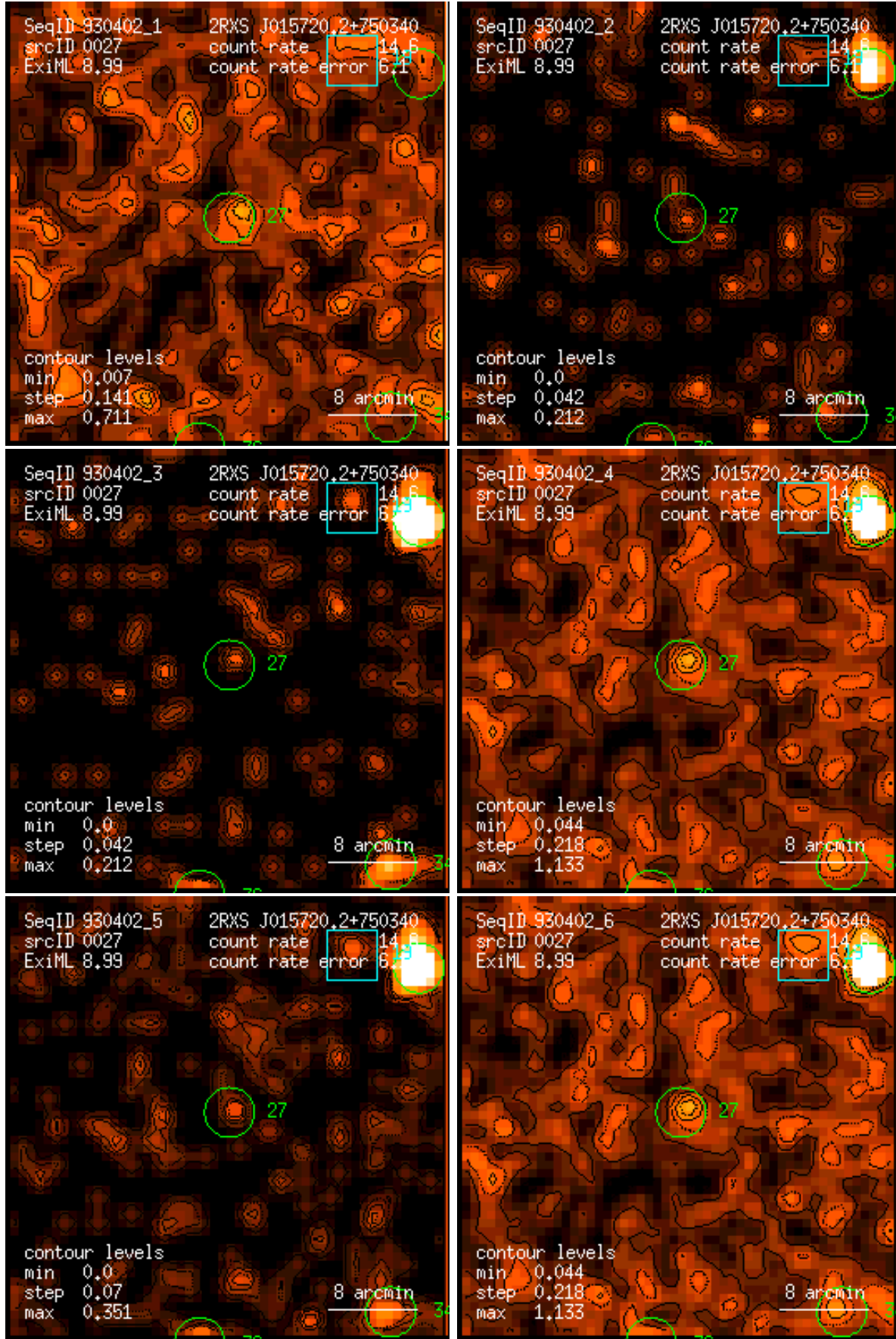
Figure 27: RASS 930402: detection 0027: band rate images, Gaussian filter: (1) PSPC channels 11 – 41, (2) 52 – 90, (3) 91 – 201, (4) 11 – 235, (5) 52 – 201, (6) 11 – 201. Broad band rates in counts/ks. Band rate contour levels in counts/ks/arcmin 2 .
