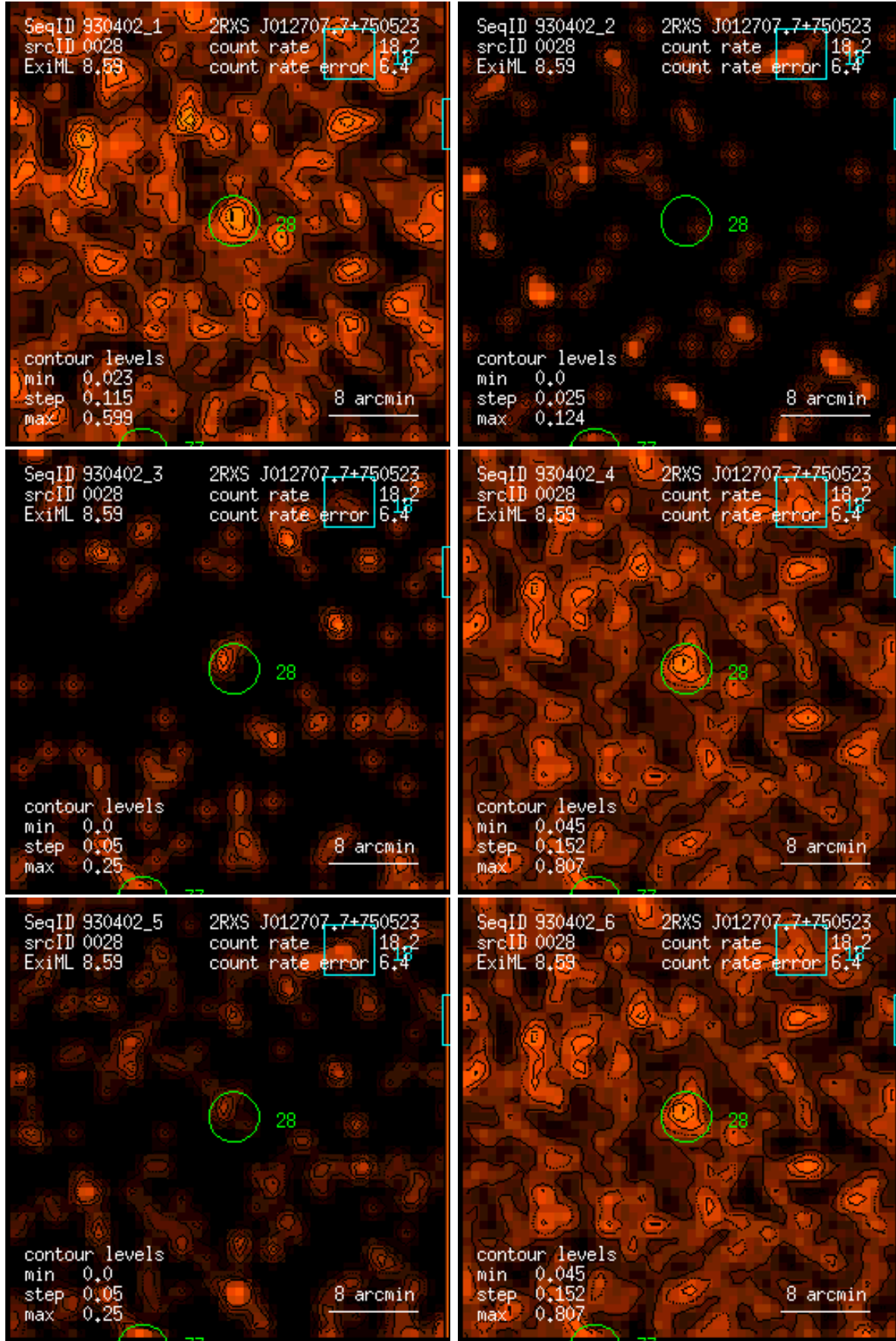
Figure 28: RASS 930402: detection 0028: band rate images, Gaussian filter: (1) PSPC channels 11 – 41, (2) 52 – 90, (3) 91 – 201, (4) 11 – 235, (5) 52 – 201, (6) 11 – 201. Broad band rates in counts/ks. Band rate contour levels in counts/ks/arcmin 2 .
