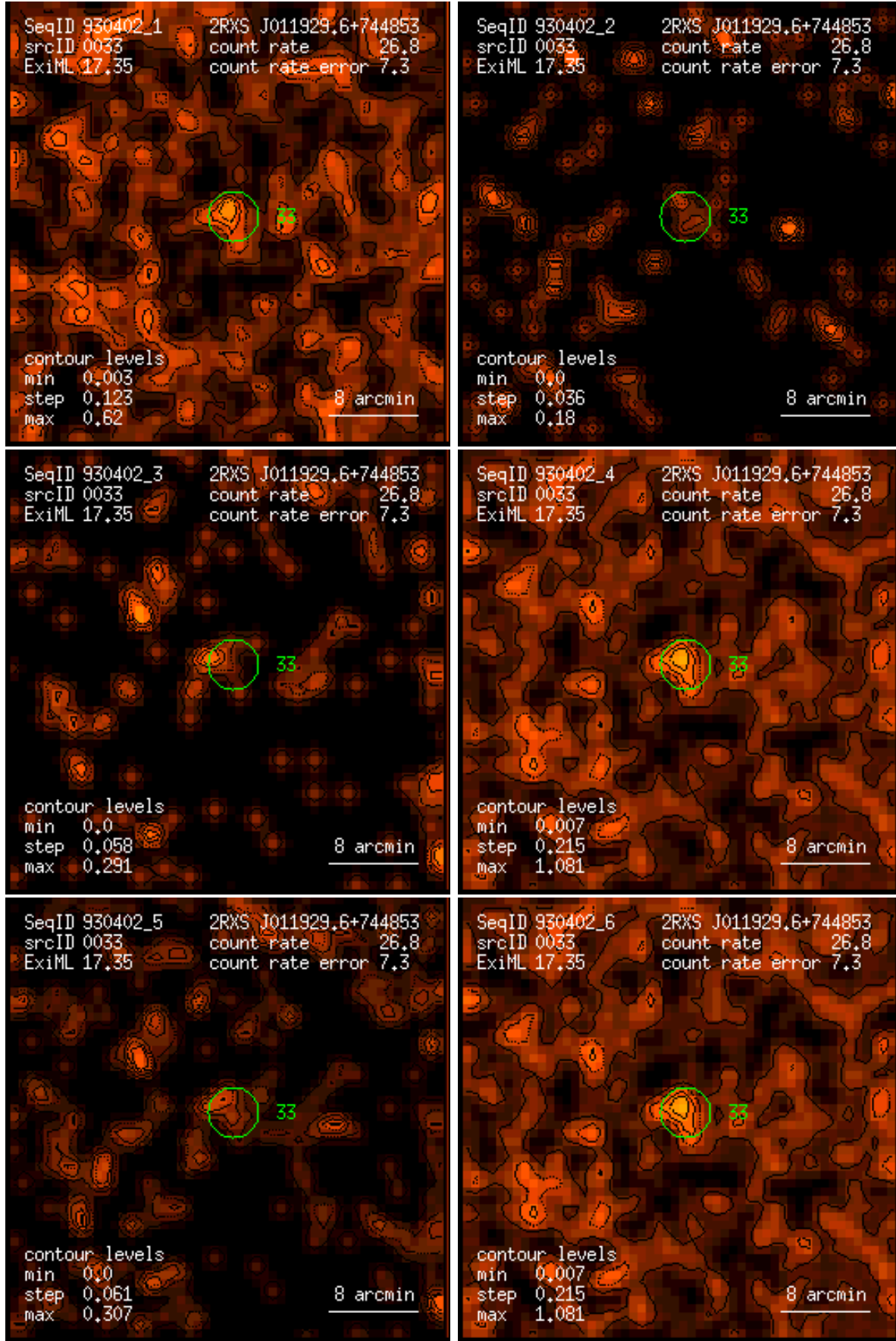
Figure 33: RASS 930402: detection 0033: band rate images, Gaussian filter: (1) PSPC channels 11 – 41, (2) 52 – 90, (3) 91 – 201, (4) 11 – 235, (5) 52 – 201, (6) 11 – 201. Broad band rates in counts/ks. Band rate contour levels in counts/ks/arcmin 2 .
