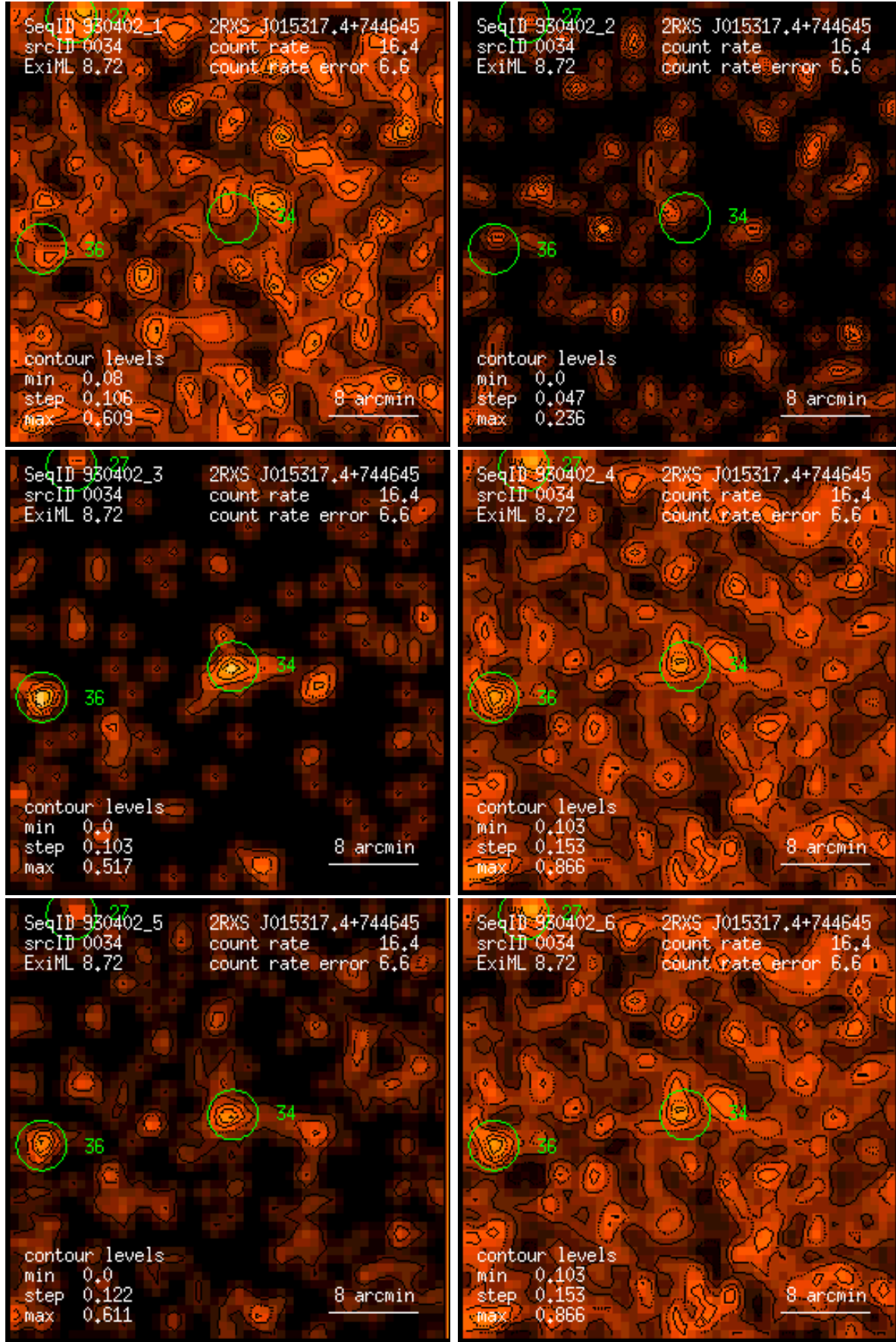
Figure 34: RASS 930402: detection 0034: band rate images, Gaussian filter: (1) PSPC channels 11 – 41, (2) 52 – 90, (3) 91 – 201, (4) 11 – 235, (5) 52 – 201, (6) 11 – 201. Broad band rates in counts/ks. Band rate contour levels in counts/ks/arcmin 2 .
