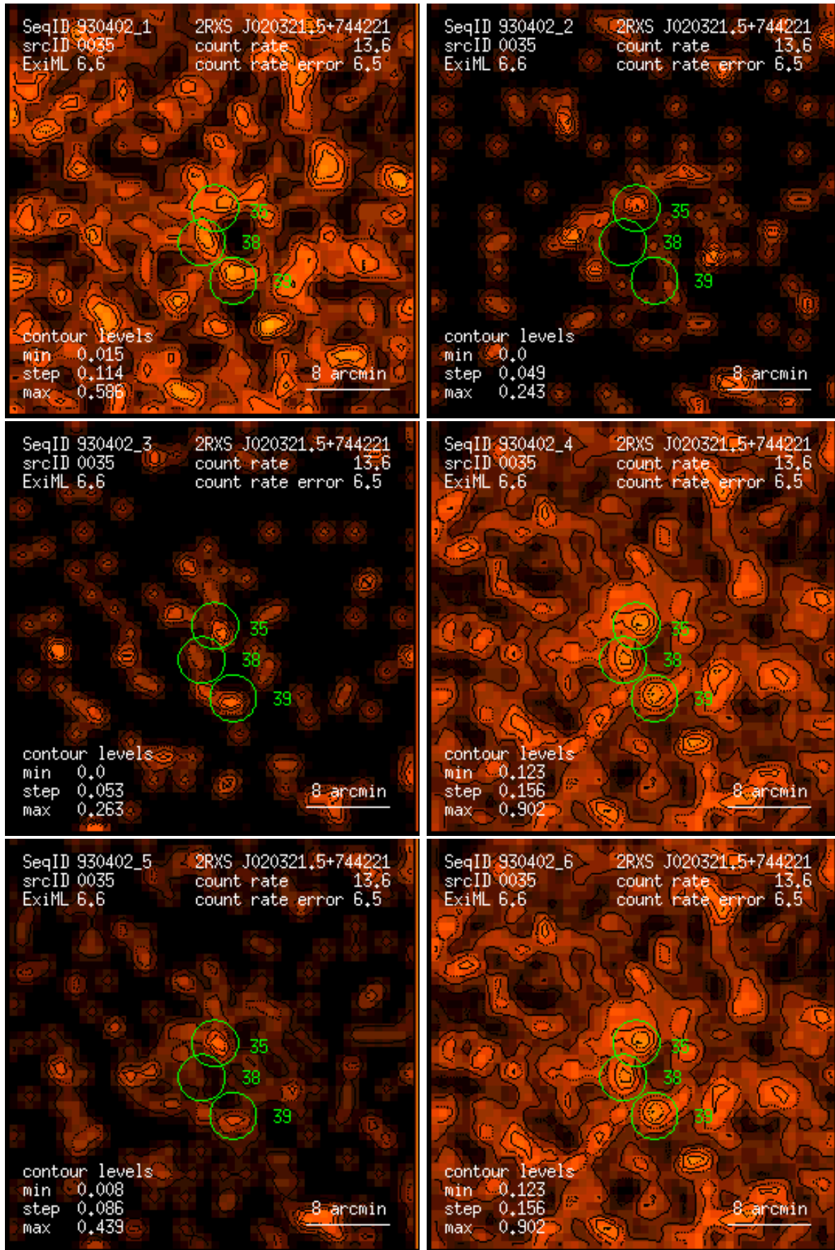
Figure 35: RASS 930402: detection 0035: band rate images, Gaussian filter: (1) PSPC channels 11 – 41, (2) 52 – 90, (3) 91 – 201, (4) 11 – 235, (5) 52 – 201, (6) 11 – 201. Broad band rates in counts/ks. Band rate contour levels in counts/ks/arcmin 2 .
