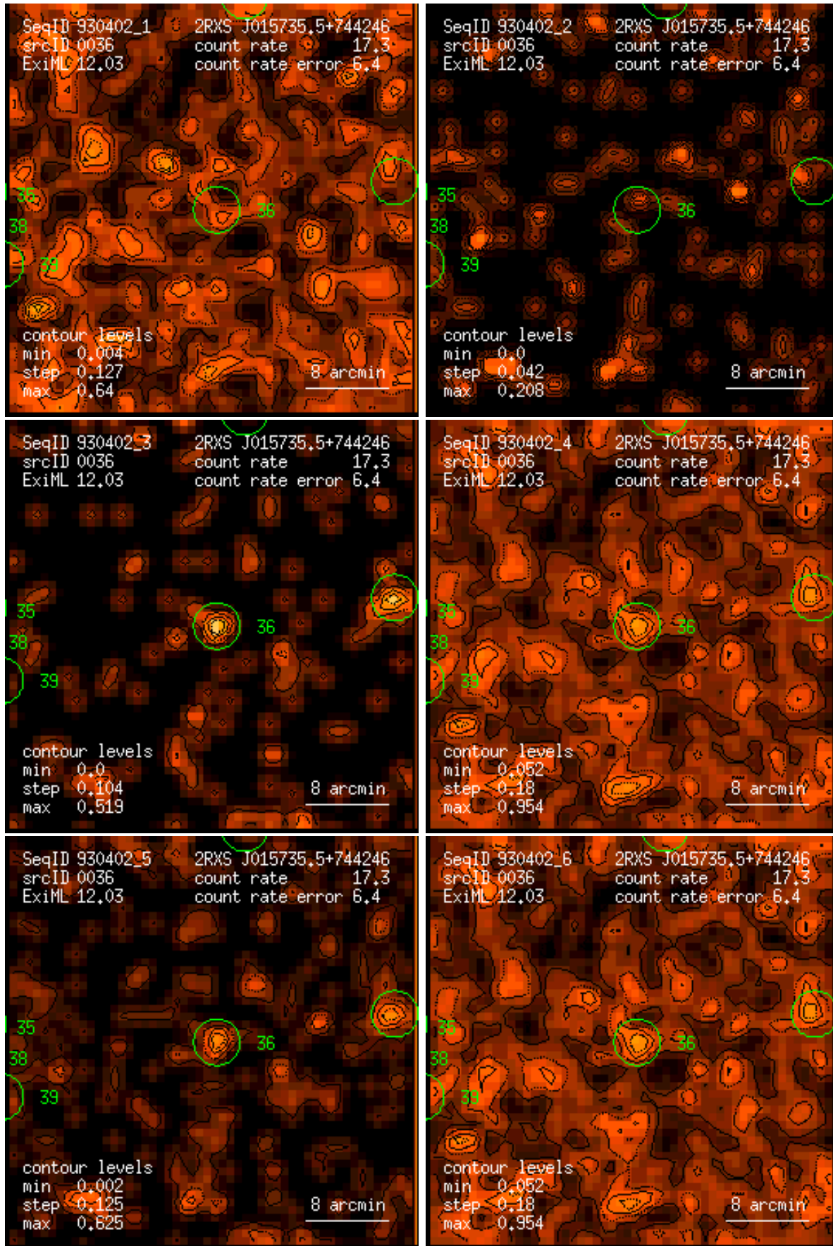
Figure 36: RASS 930402: detection 0036: band rate images, Gaussian filter: (1) PSPC channels 11 – 41, (2) 52 – 90, (3) 91 – 201, (4) 11 – 235, (5) 52 – 201, (6) 11 – 201. Broad band rates in counts/ks. Band rate contour levels in counts/ks/arcmin 2 .
