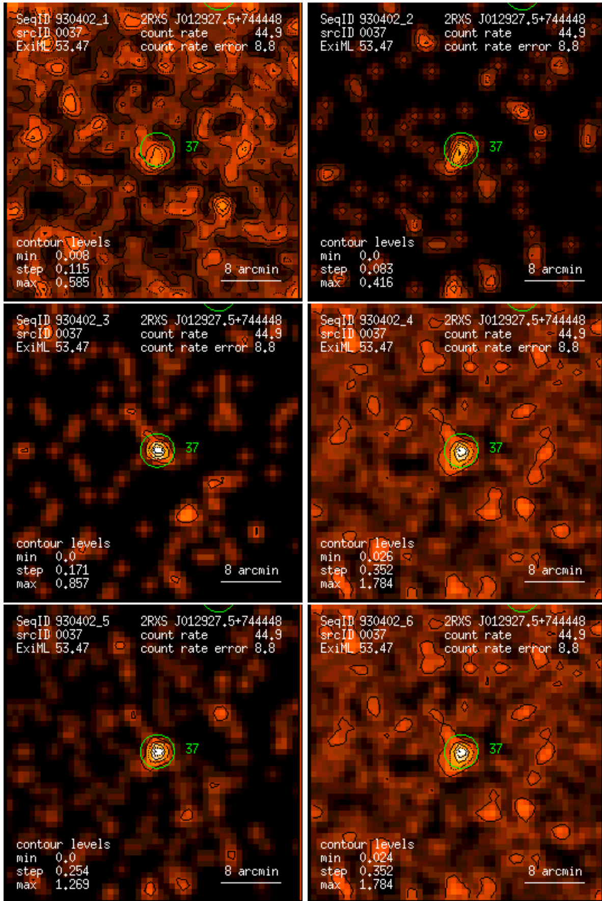
Figure 37: RASS 930402: detection 0037: band rate images, Gaussian filter: (1) PSPC channels 11 – 41, (2) 52 – 90, (3) 91 – 201, (4) 11 – 235, (5) 52 – 201, (6) 11 – 201. Broad band rates in counts/ks. Band rate contour levels in counts/ks/arcmin 2 .
