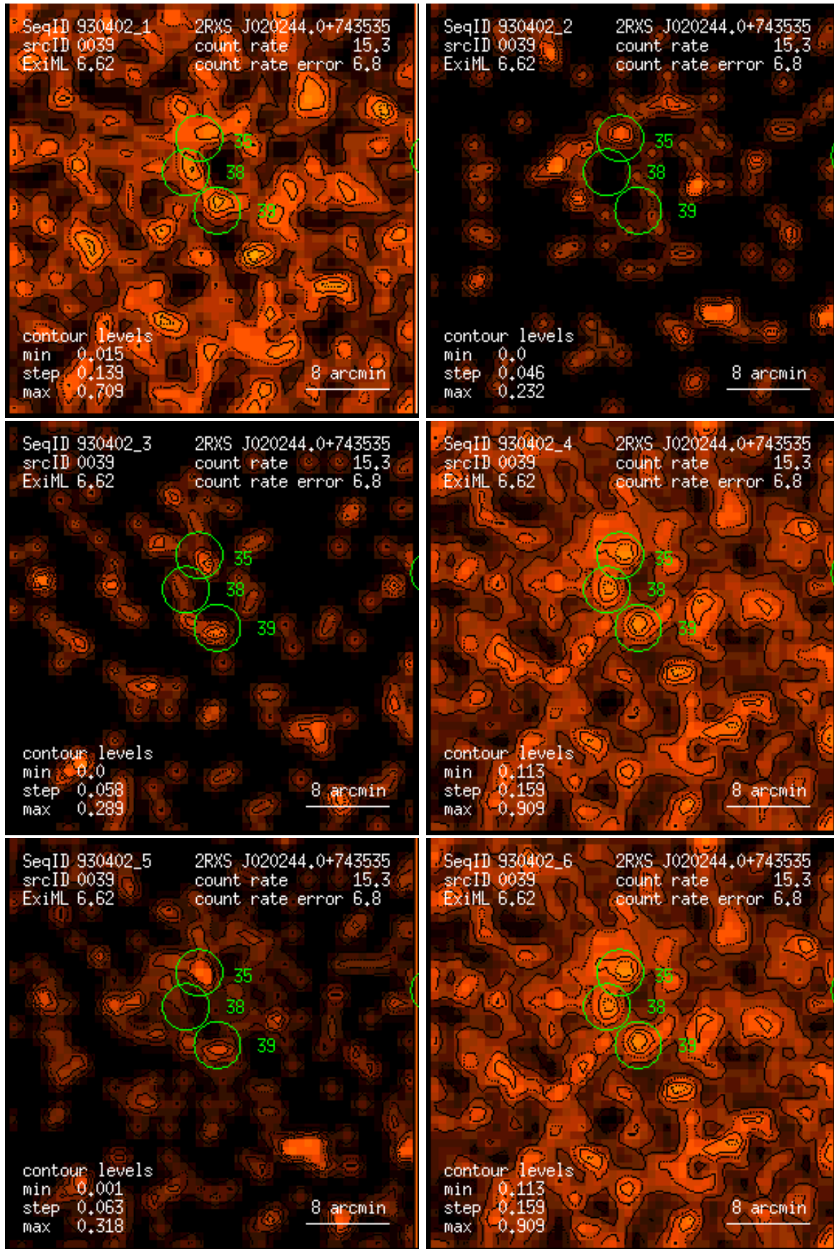
Figure 39: RASS 930402: detection 0039: band rate images, Gaussian filter: (1) PSPC channels 11 – 41, (2) 52 – 90, (3) 91 – 201, (4) 11 – 235, (5) 52 – 201, (6) 11 – 201. Broad band rates in counts/ks. Band rate contour levels in counts/ks/arcmin 2 .
