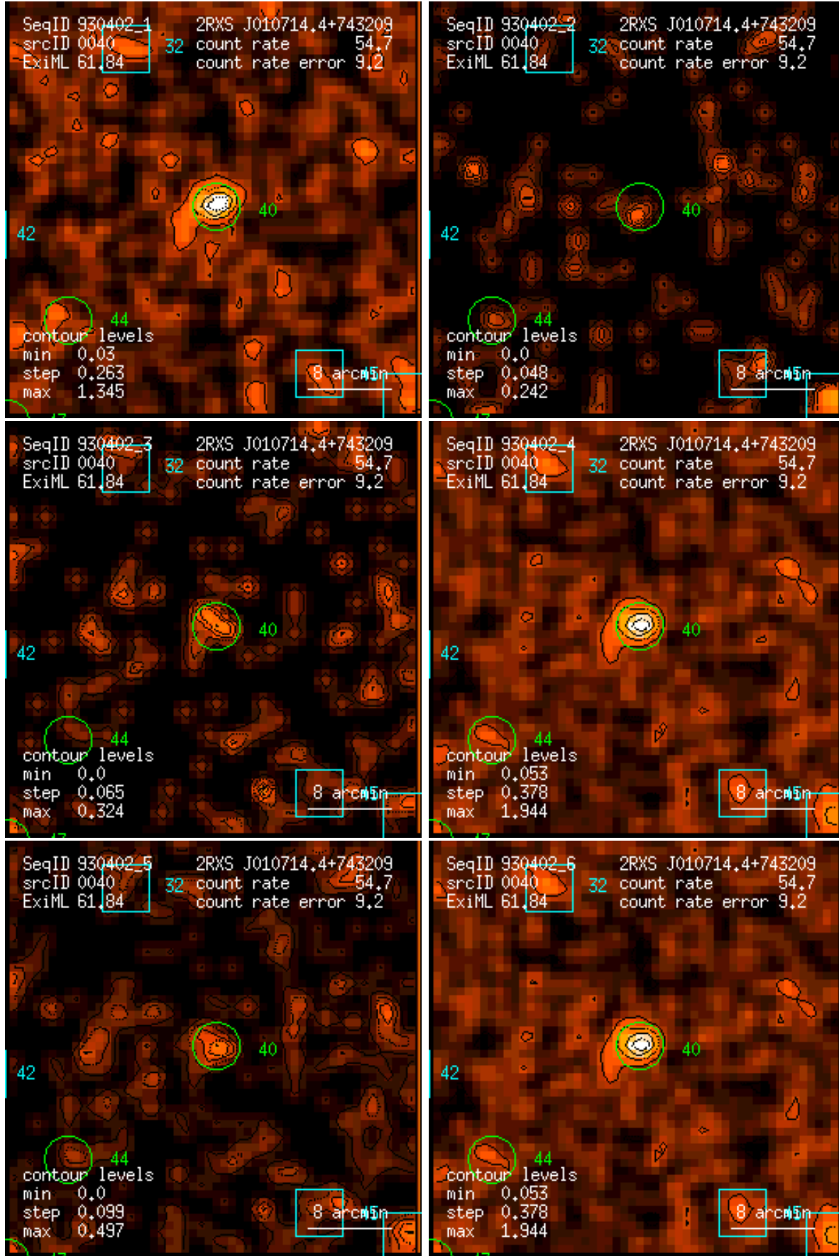
Figure 40: RASS 930402: detection 0040: band rate images, Gaussian filter: (1) PSPC channels 11 – 41, (2) 52 – 90, (3) 91 – 201, (4) 11 – 235, (5) 52 – 201, (6) 11 – 201. Broad band rates in counts/ks. Band rate contour levels in counts/ks/arcmin 2 .
