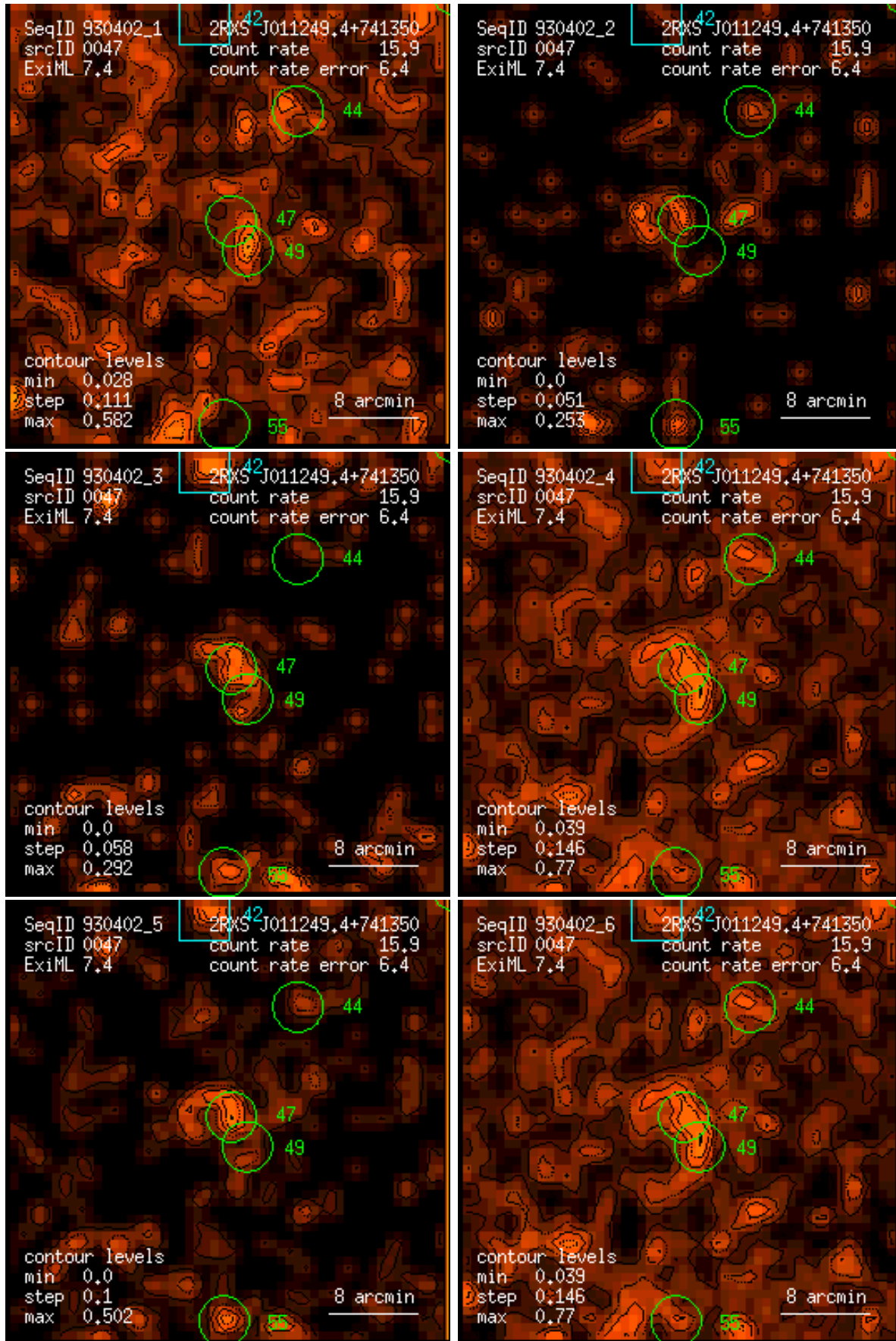
Figure 47: RASS 930402: detection 0047: band rate images, Gaussian filter: (1) PSPC channels 11 – 41, (2) 52 – 90, (3) 91 – 201, (4) 11 – 235, (5) 52 – 201, (6) 11 – 201. Broad band rates in counts/ks. Band rate contour levels in counts/ks/arcmin 2 .
