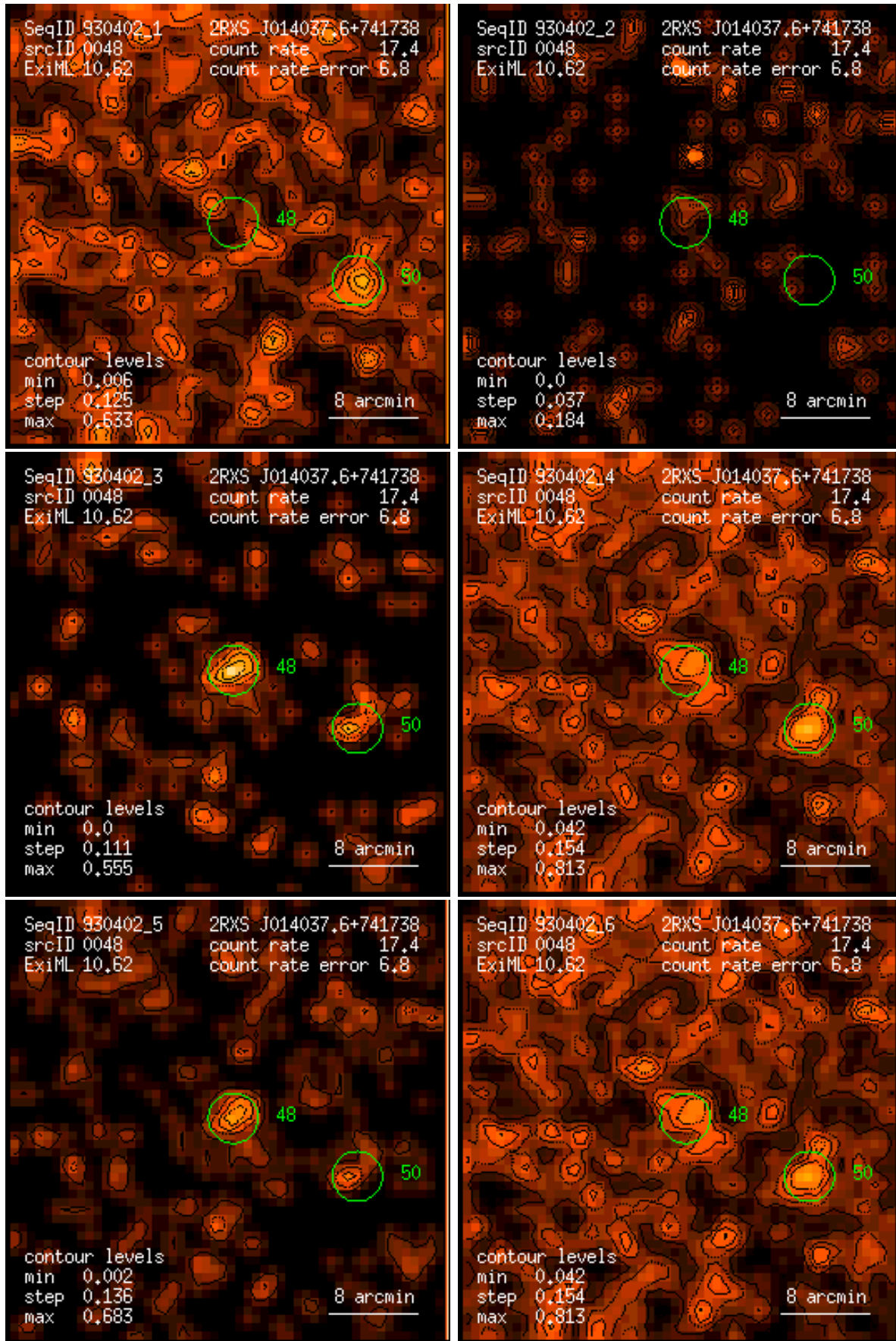
Figure 48: RASS 930402: detection 0048: band rate images, Gaussian filter: (1) PSPC channels 11 – 41, (2) 52 – 90, (3) 91 – 201, (4) 11 – 235, (5) 52 – 201, (6) 11 – 201. Broad band rates in counts/ks. Band rate contour levels in counts/ks/arcmin 2 .
