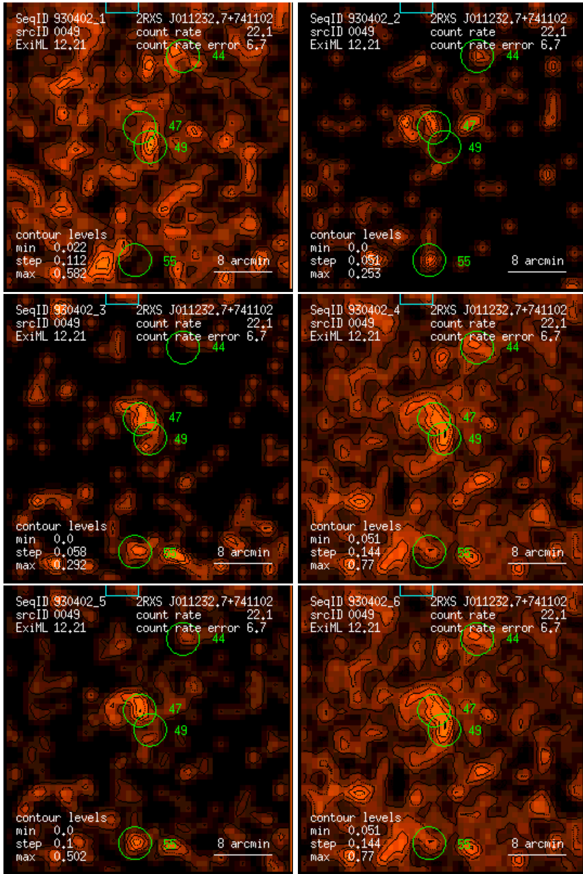
Figure 49: RASS 930402: detection 0049: band rate images, Gaussian filter: (1) PSPC channels 11 – 41, (2) 52 – 90, (3) 91 – 201, (4) 11 – 235, (5) 52 – 201, (6) 11 – 201. Broad band rates in counts/ks. Band rate contour levels in counts/ks/arcmin 2 .
