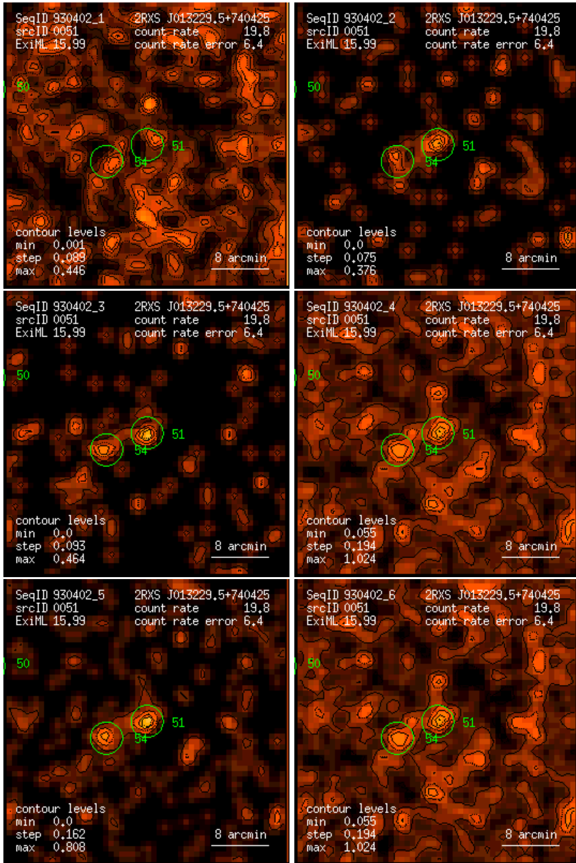
Figure 51: RASS 930402: detection 0051: band rate images, Gaussian filter: (1) PSPC channels 11 – 41, (2) 52 – 90, (3) 91 – 201, (4) 11 – 235, (5) 52 – 201, (6) 11 – 201. Broad band rates in counts/ks. Band rate contour levels in counts/ks/arcmin 2 .
