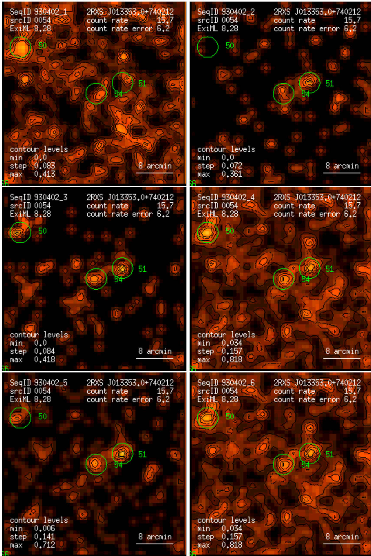
Figure 54: RASS 930402: detection 0054: band rate images, Gaussian filter: (1) PSPC channels 11 – 41, (2) 52 – 90, (3) 91 – 201, (4) 11 – 235, (5) 52 – 201, (6) 11 – 201. Broad band rates in counts/ks. Band rate contour levels in counts/ks/arcmin 2 .
