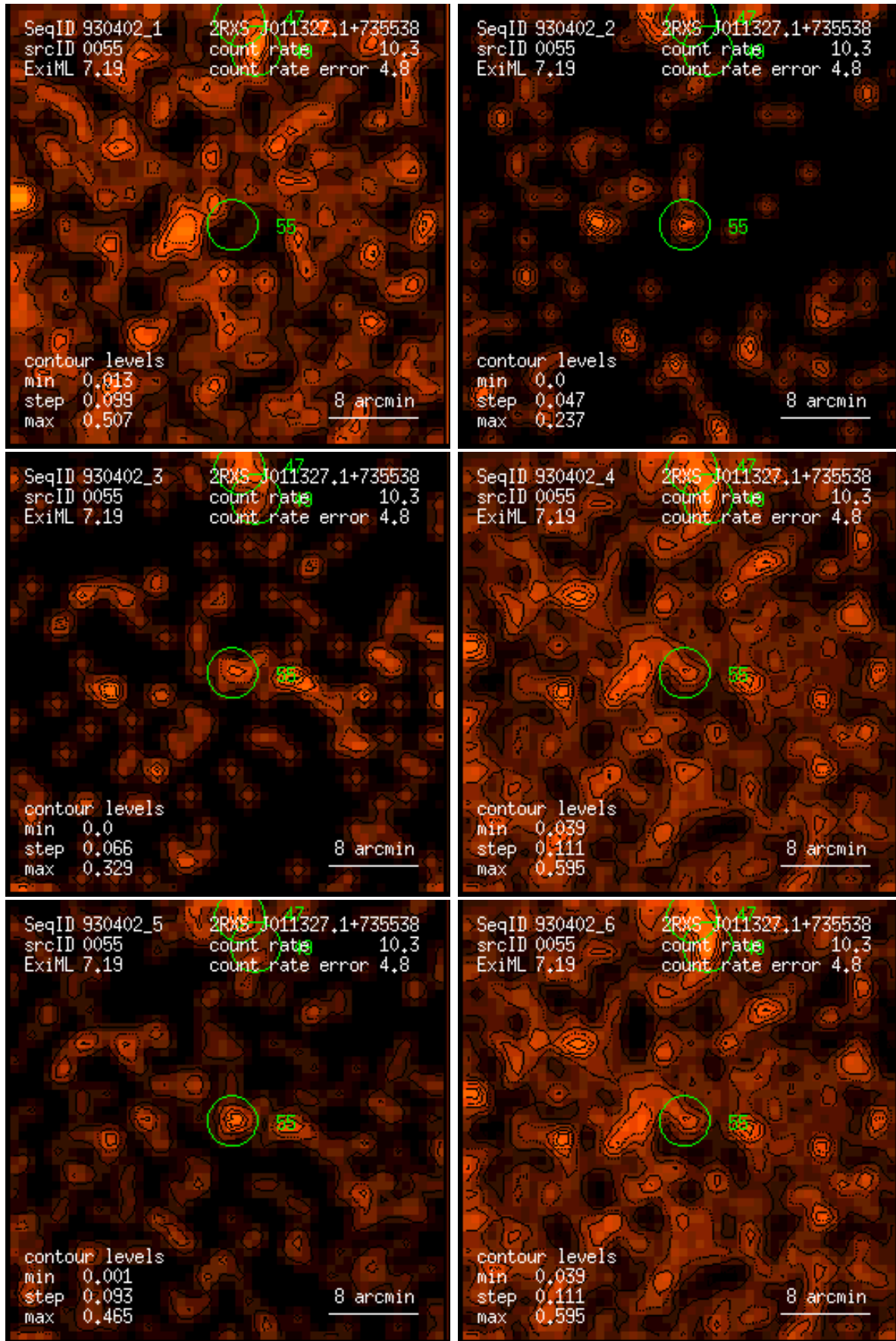
Figure 55: RASS 930402: detection 0055: band rate images, Gaussian filter: (1) PSPC channels 11 – 41, (2) 52 – 90, (3) 91 – 201, (4) 11 – 235, (5) 52 – 201, (6) 11 – 201. Broad band rates in counts/ks. Band rate contour levels in counts/ks/arcmin 2 .
