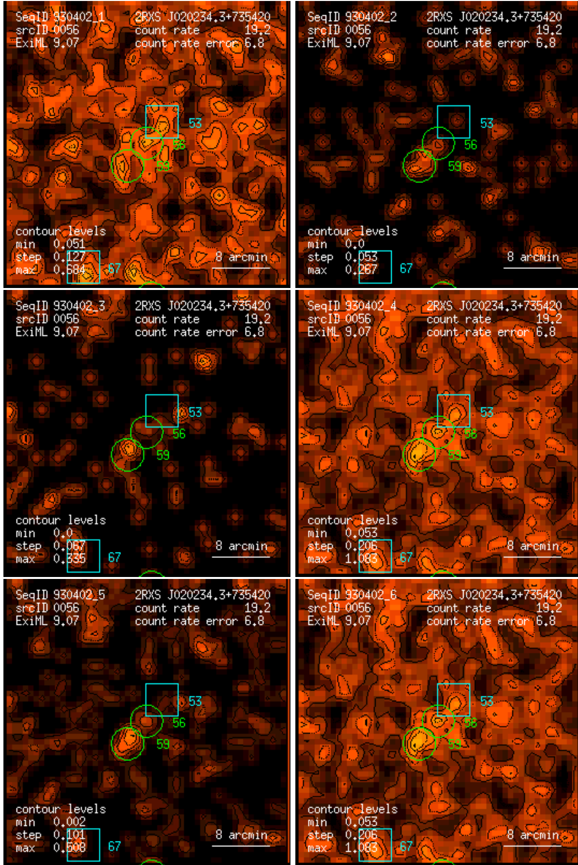
Figure 56: RASS 930402: detection 0056: band rate images, Gaussian filter: (1) PSPC channels 11 – 41, (2) 52 – 90, (3) 91 – 201, (4) 11 – 235, (5) 52 – 201, (6) 11 – 201. Broad band rates in counts/ks. Band rate contour levels in counts/ks/arcmin 2 .
