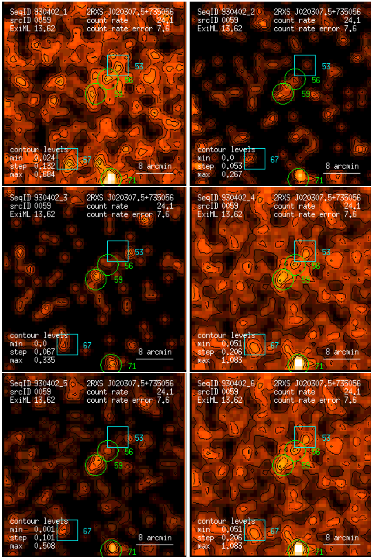
Figure 59: RASS 930402: detection 0059: band rate images, Gaussian filter: (1) PSPC channels 11 – 41, (2) 52 – 90, (3) 91 – 201, (4) 11 – 235, (5) 52 – 201, (6) 11 – 201. Broad band rates in counts/ks. Band rate contour levels in counts/ks/arcmin 2 .
