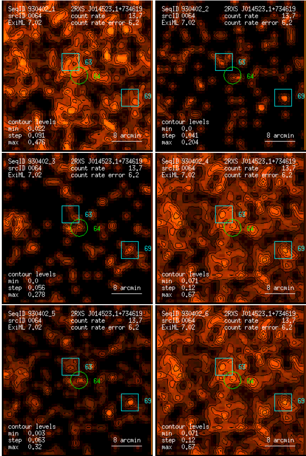
Figure 64: RASS 930402: detection 0064: band rate images, Gaussian filter: (1) PSPC channels 11 – 41, (2) 52 – 90, (3) 91 – 201, (4) 11 – 235, (5) 52 – 201, (6) 11 – 201. Broad band rates in counts/ks. Band rate contour levels in counts/ks/arcmin 2 .
