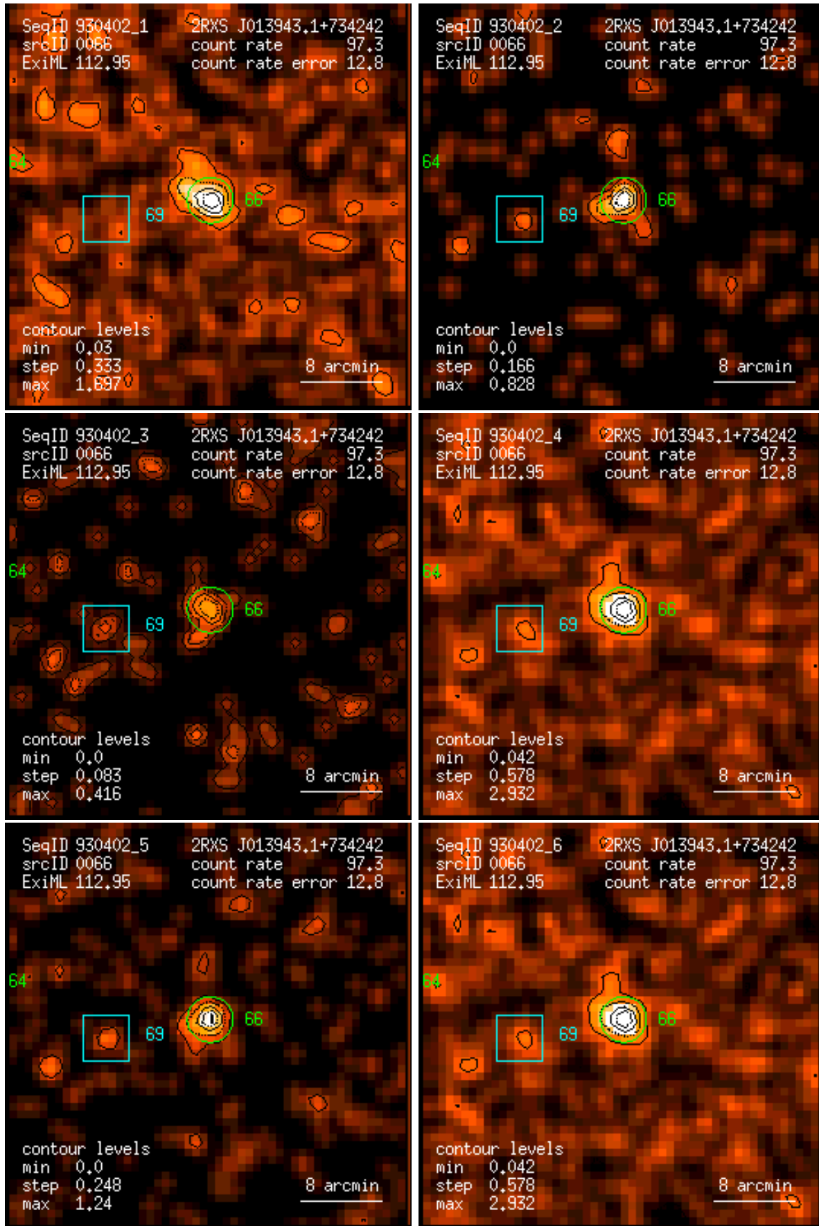
Figure 66: RASS 930402: detection 0066: band rate images, Gaussian filter: (1) PSPC channels 11 – 41, (2) 52 – 90, (3) 91 – 201, (4) 11 – 235, (5) 52 – 201, (6) 11 – 201. Broad band rates in counts/ks. Band rate contour levels in counts/ks/arcmin 2 .
