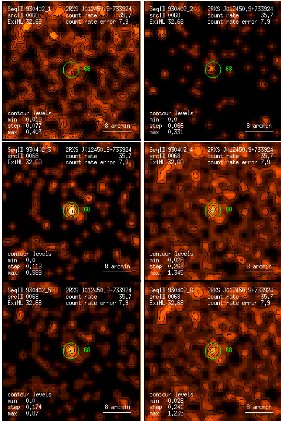
Figure 68: RASS 930402: detection 0068: band rate images, Gaussian filter: (1) PSPC channels 11 – 41, (2) 52 – 90, (3) 91 – 201, (4) 11 – 235, (5) 52 – 201, (6) 11 – 201. Broad band rates in counts/ks. Band rate contour levels in counts/ks/arcmin 2 .
