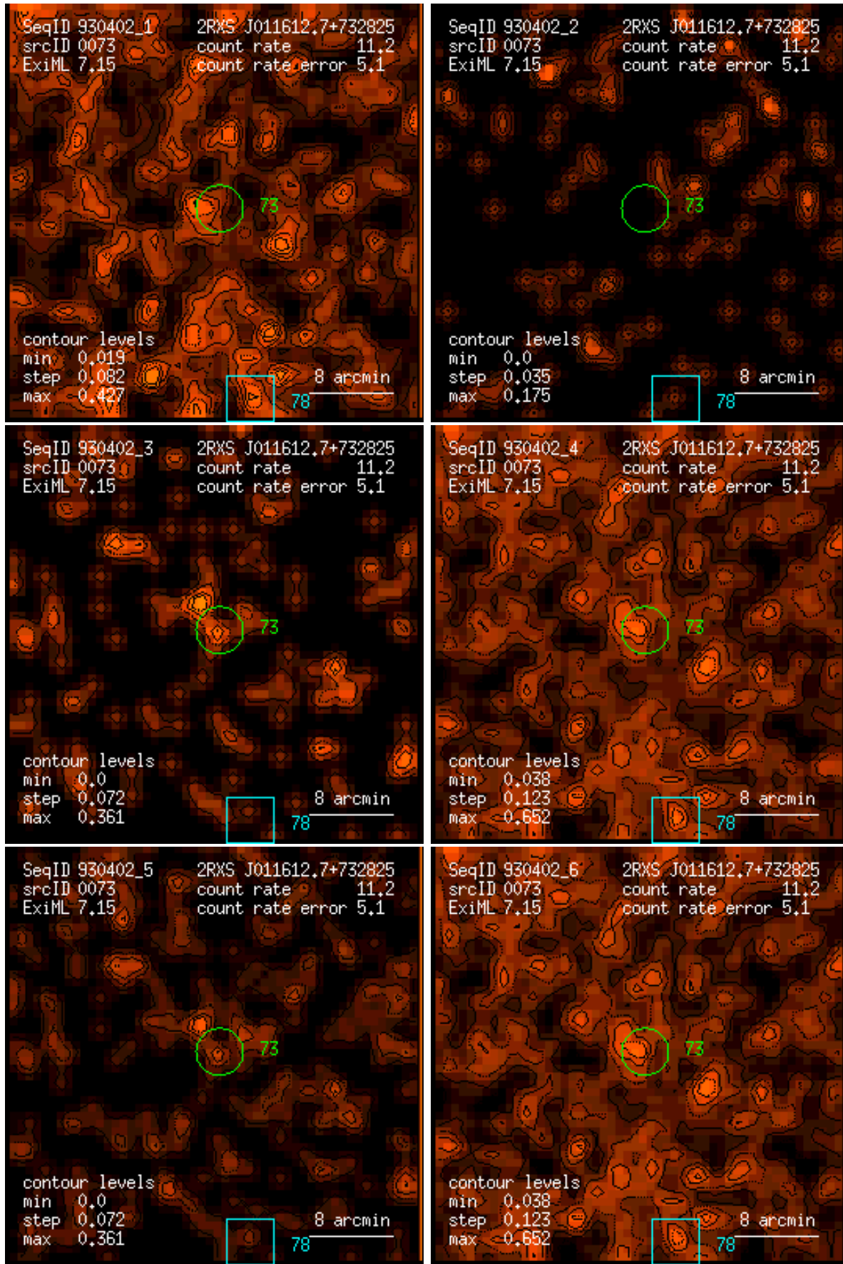
Figure 73: RASS 930402: detection 0073: band rate images, Gaussian filter: (1) PSPC channels 11 – 41, (2) 52 – 90, (3) 91 – 201, (4) 11 – 235, (5) 52 – 201, (6) 11 – 201. Broad band rates in counts/ks. Band rate contour levels in counts/ks/arcmin 2 .
