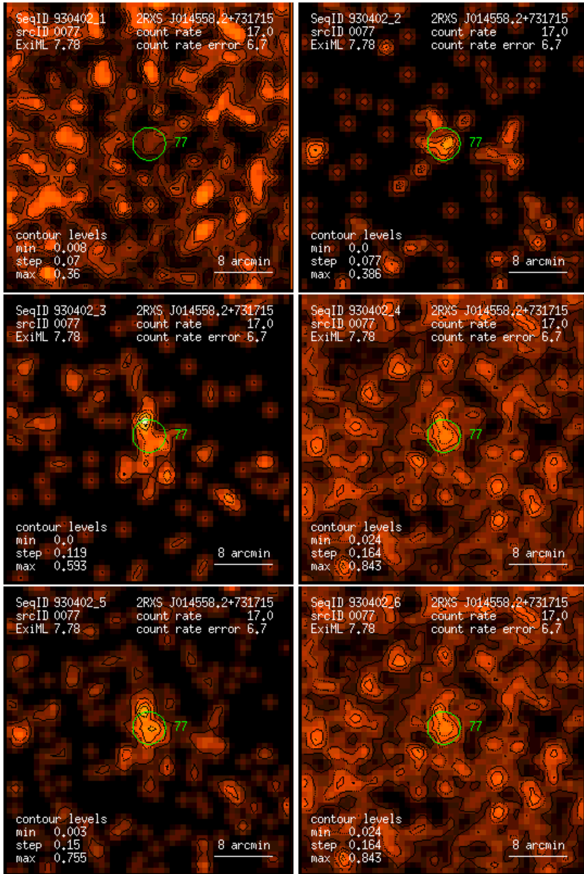
Figure 77: RASS 930402: detection 0077: band rate images, Gaussian filter: (1) PSPC channels 11 – 41, (2) 52 – 90, (3) 91 – 201, (4) 11 – 235, (5) 52 – 201, (6) 11 – 201. Broad band rates in counts/ks. Band rate contour levels in counts/ks/arcmin 2 .
