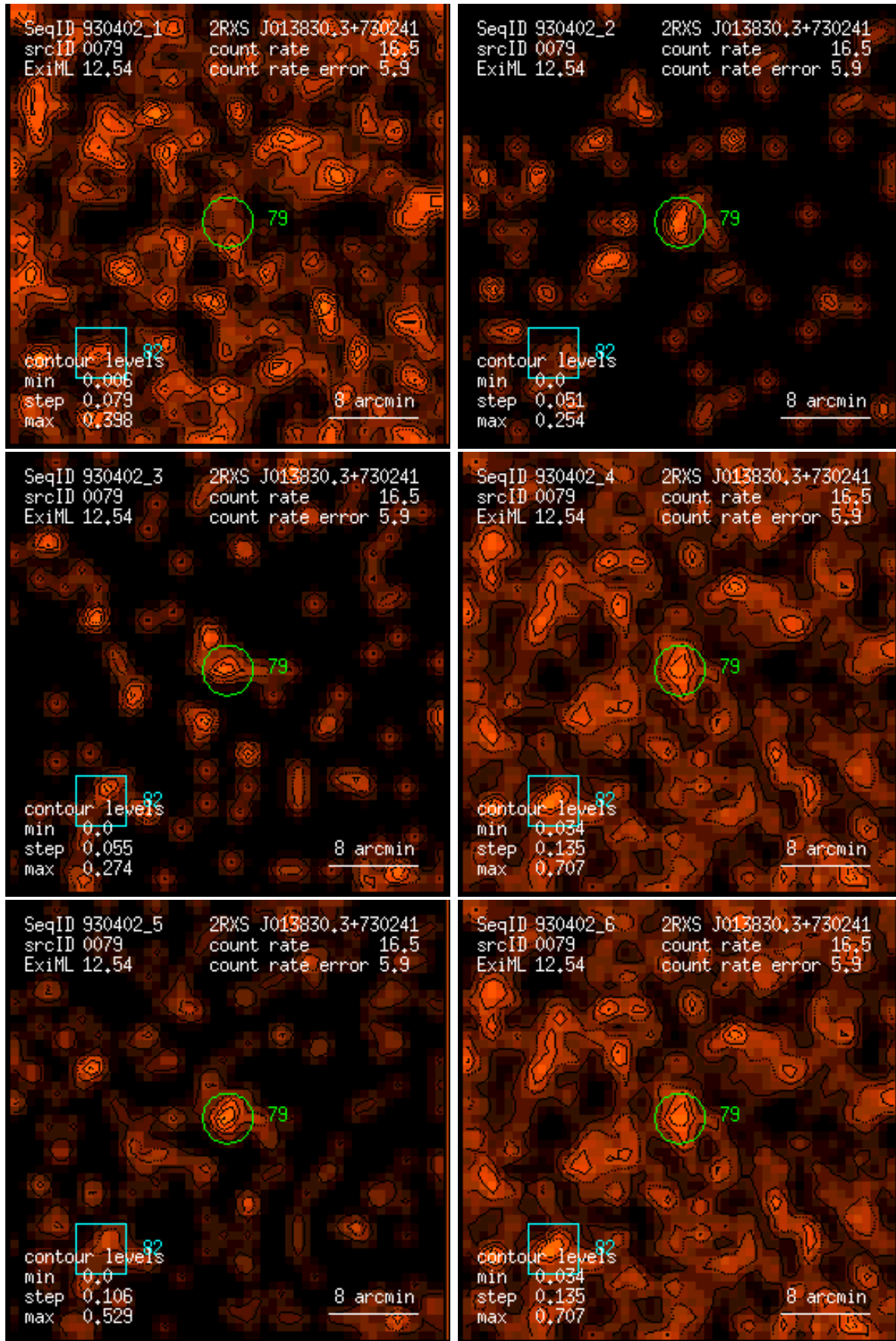
Figure 79: RASS 930402: detection 0079: band rate images, Gaussian filter: (1) PSPC channels 11 – 41, (2) 52 – 90, (3) 91 – 201, (4) 11 – 235, (5) 52 – 201, (6) 11 – 201. Broad band rates in counts/ks. Band rate contour levels in counts/ks/arcmin 2 .
