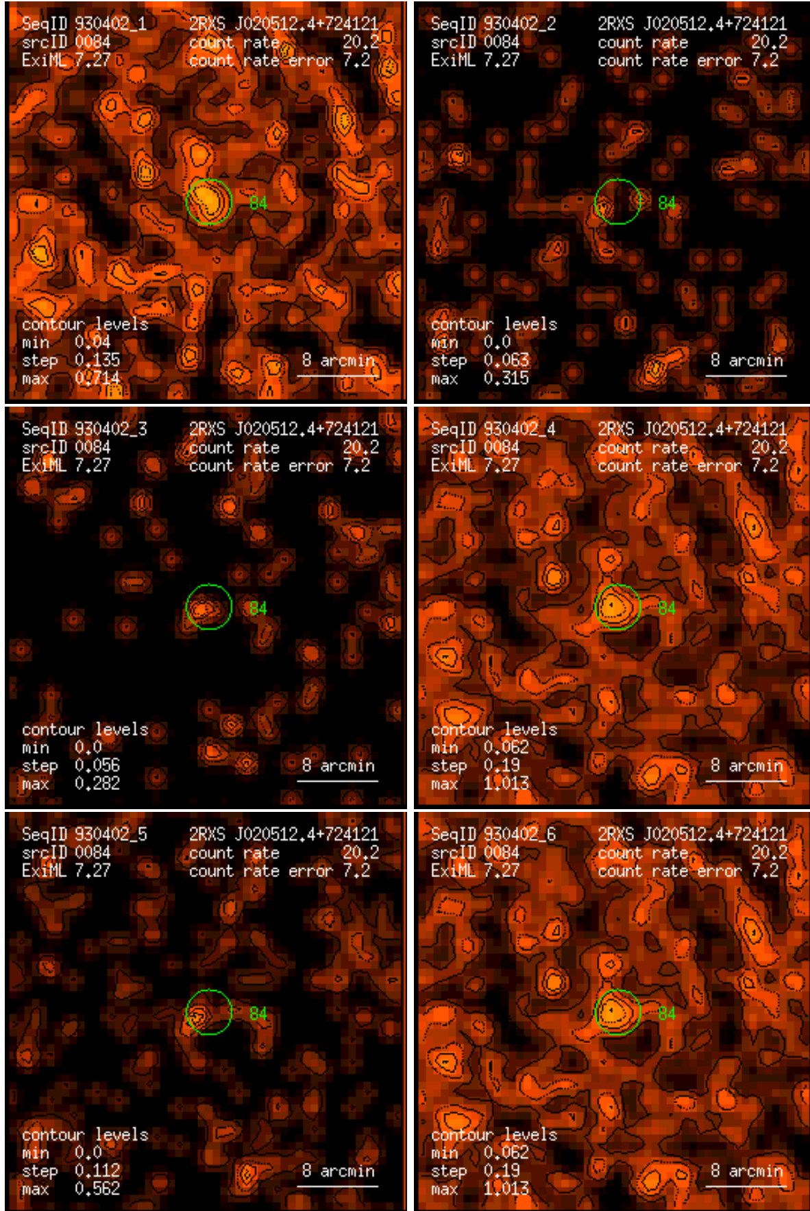
Figure 84: RASS 930402: detection 0084: band rate images, Gaussian filter: (1) PSPC channels 11 – 41, (2) 52 – 90, (3) 91 – 201, (4) 11 – 235, (5) 52 – 201, (6) 11 – 201. Broad band rates in counts/ks. Band rate contour levels in counts/ks/arcmin 2 .
