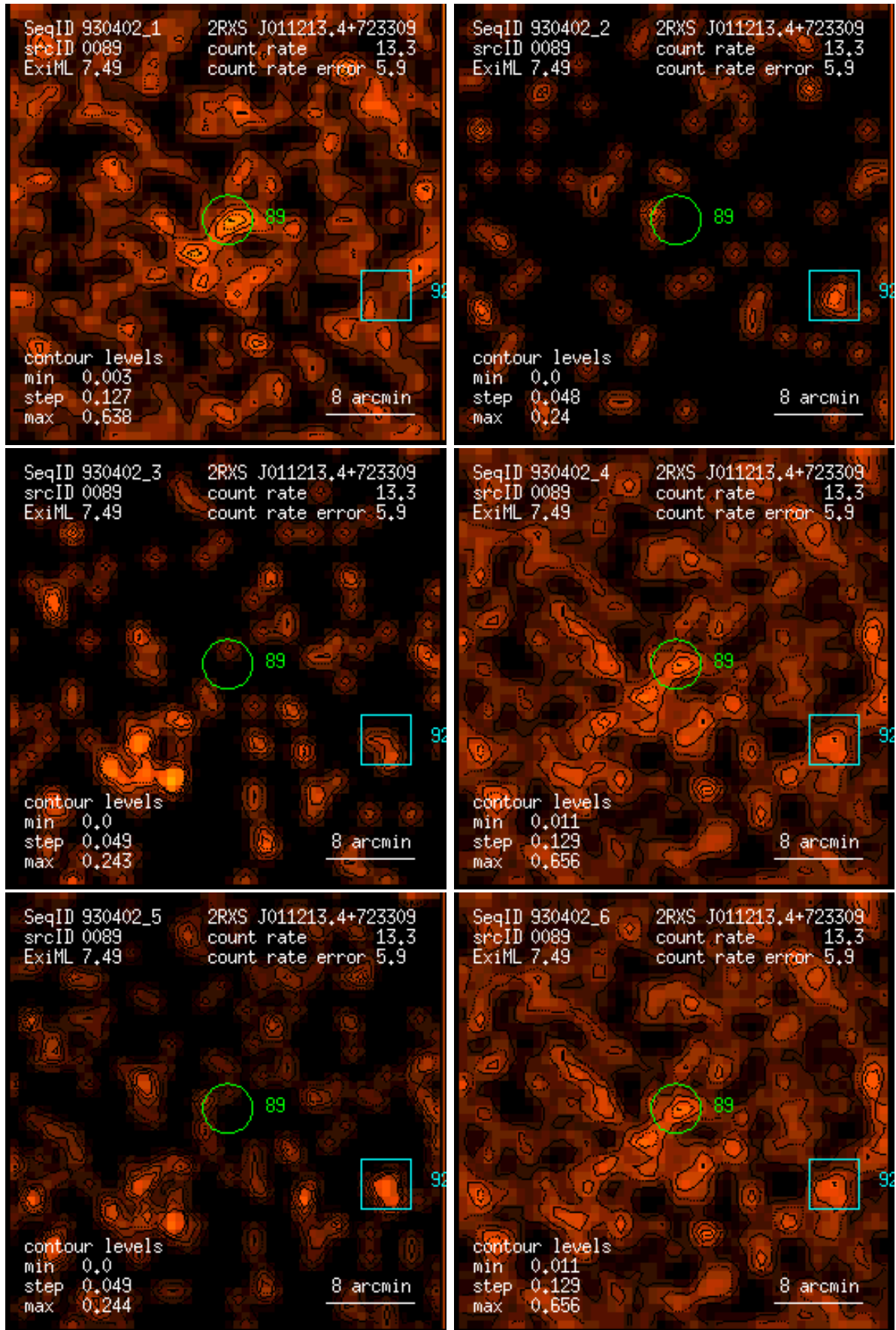
Figure 89: RASS 930402: detection 0089: band rate images, Gaussian filter: (1) PSPC channels 11 – 41, (2) 52 – 90, (3) 91 – 201, (4) 11 – 235, (5) 52 – 201, (6) 11 – 201. Broad band rates in counts/ks. Band rate contour levels in counts/ks/arcmin 2 .
