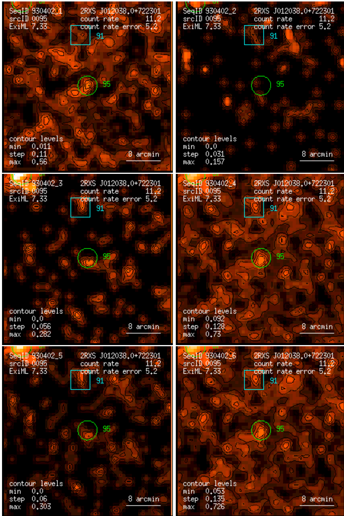
Figure 95: RASS 930402: detection 0095: band rate images, Gaussian filter: (1) PSPC channels 11 – 41, (2) 52 – 90, (3) 91 – 201, (4) 11 – 235, (5) 52 – 201, (6) 11 – 201. Broad band rates in counts/ks. Band rate contour levels in counts/ks/arcmin 2 .
