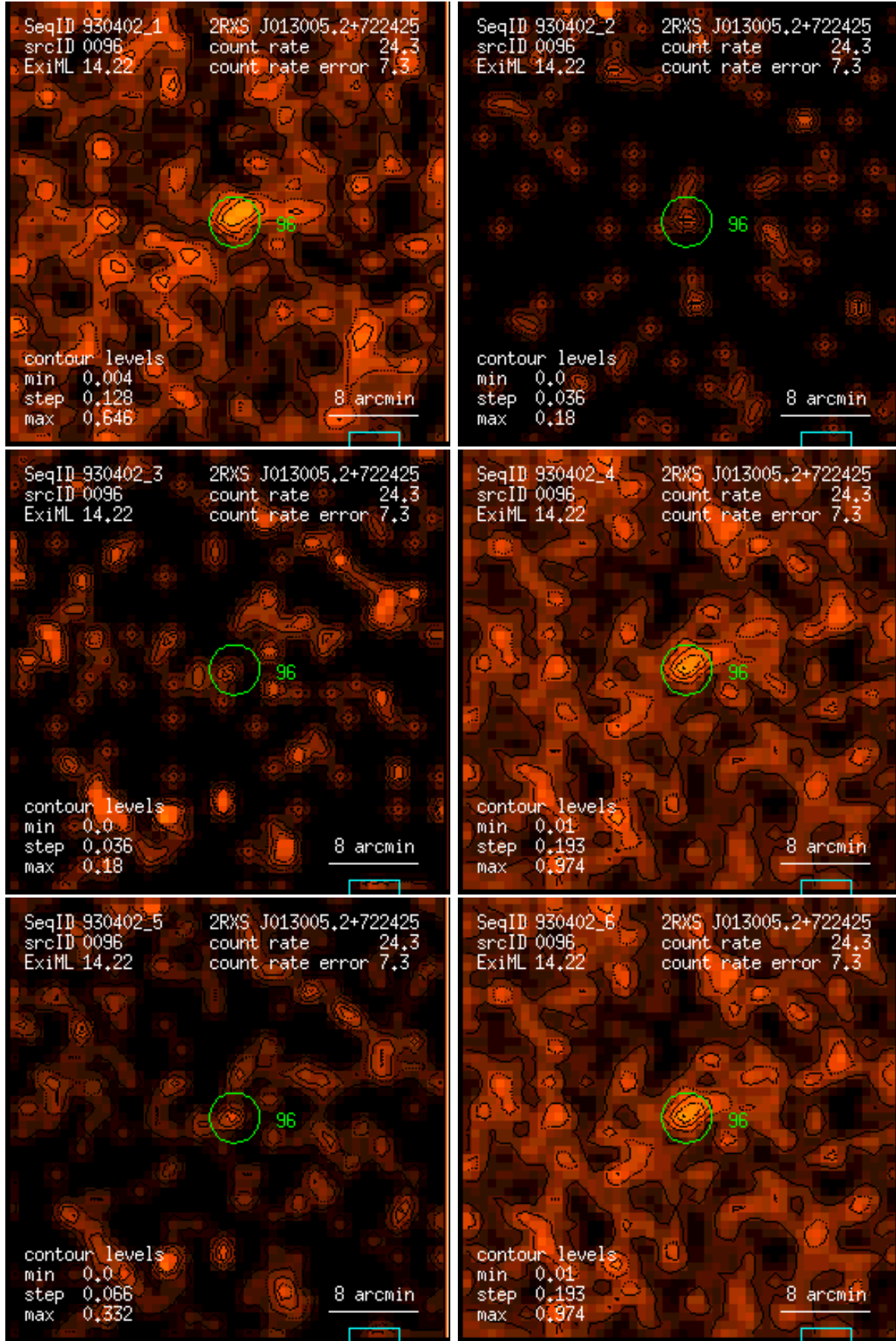
Figure 96: RASS 930402: detection 0096: band rate images, Gaussian filter: (1) PSPC channels 11 – 41, (2) 52 – 90, (3) 91 – 201, (4) 11 – 235, (5) 52 – 201, (6) 11 – 201. Broad band rates in counts/ks. Band rate contour levels in counts/ks/arcmin 2 .
