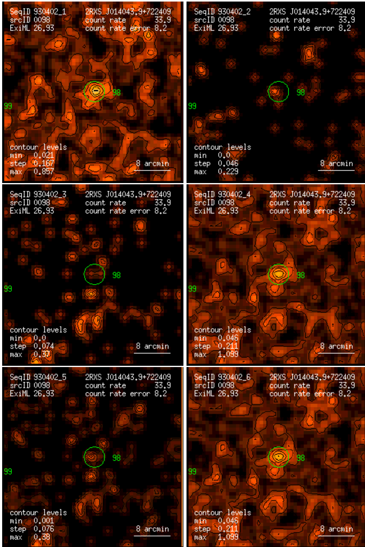
Figure 98: RASS 930402: detection 0098: band rate images, Gaussian filter: (1) PSPC channels 11 – 41, (2) 52 – 90, (3) 91 – 201, (4) 11 – 235, (5) 52 – 201, (6) 11 – 201. Broad band rates in counts/ks. Band rate contour levels in counts/ks/arcmin 2 .
