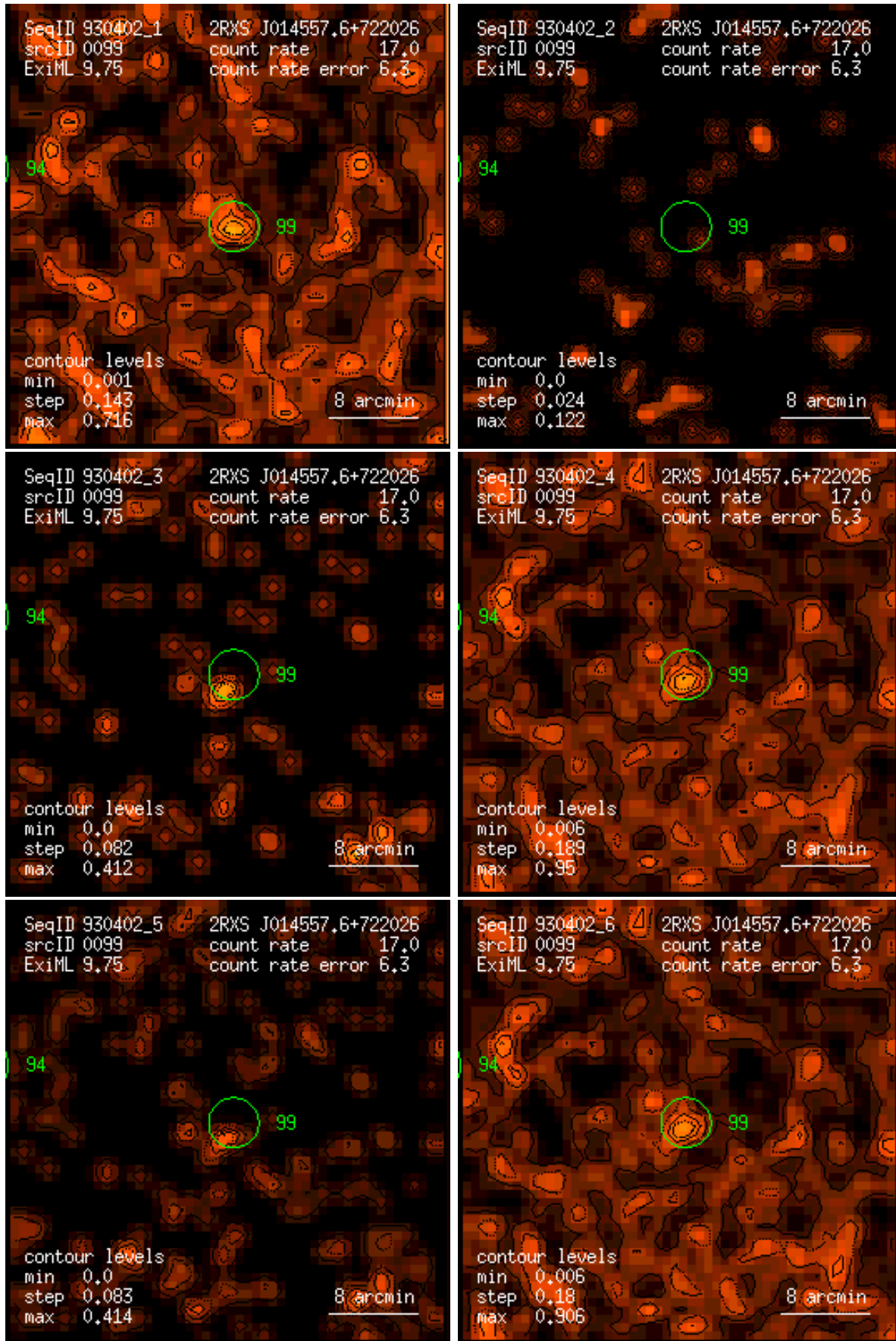
Figure 99: RASS 930402: detection 0099: band rate images, Gaussian filter: (1) PSPC channels 11 – 41, (2) 52 – 90, (3) 91 – 201, (4) 11 – 235, (5) 52 – 201, (6) 11 – 201. Broad band rates in counts/ks. Band rate contour levels in counts/ks/arcmin 2 .
