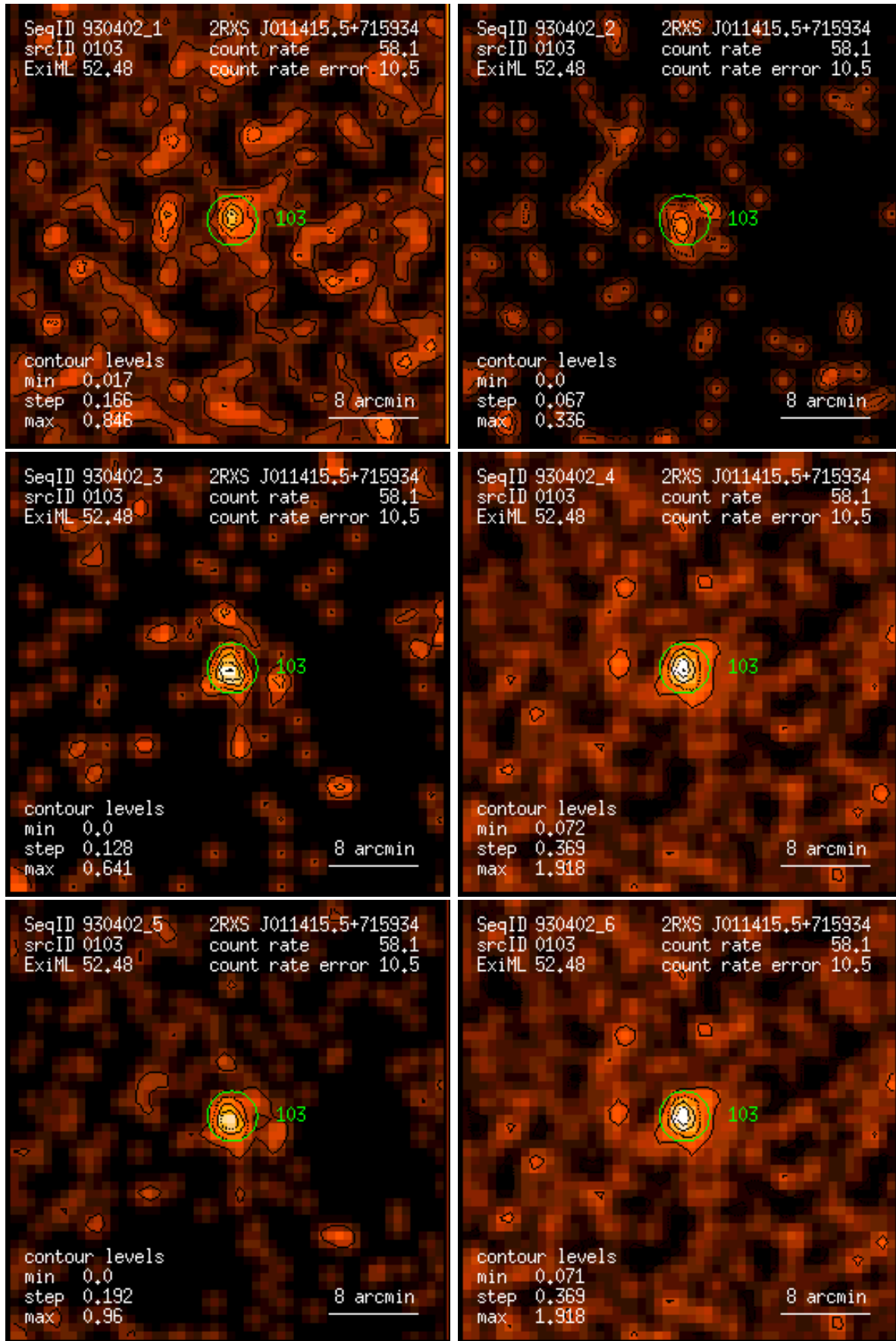
Figure 103: RASS 930402: detection 0103: band rate images, Gaussian filter: (1) PSPC channels 11 – 41, (2) 52 – 90, (3) 91 – 201, (4) 11 – 235, (5) 52 – 201, (6) 11 – 201. Broad band rates in counts/ks. Band rate contour levels in counts/ks/arcmin 2 .
