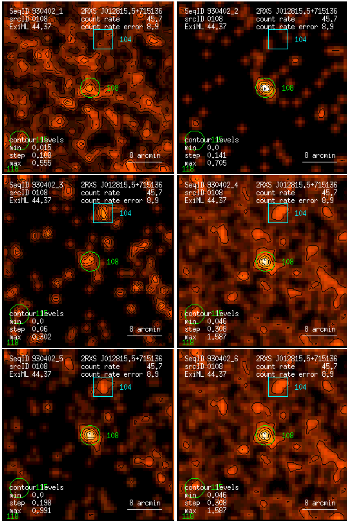
Figure 108: RASS 930402: detection 0108: band rate images, Gaussian filter: (1) PSPC channels 11 – 41, (2) 52 – 90, (3) 91 – 201, (4) 11 – 235, (5) 52 – 201, (6) 11 – 201. Broad band rates in counts/ks. Band rate contour levels in counts/ks/arcmin 2 .
